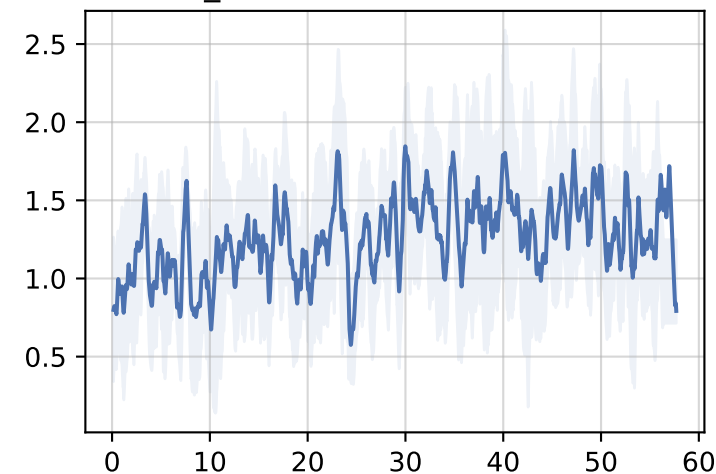
dm_control/walker-run-v0
