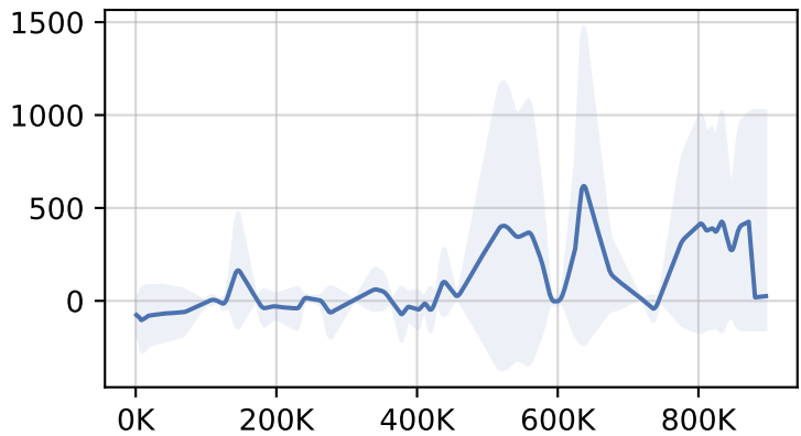
HalfCheetah-v4
