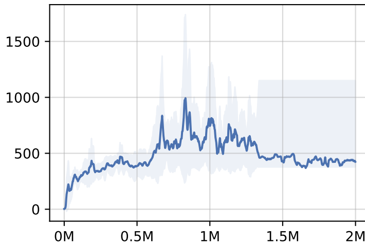
dm_control/cheetah-run-v0
