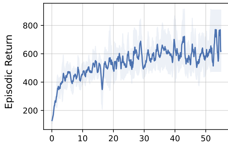
dm_control/humanoid-run-v0
