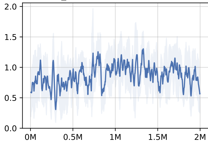
dm_control/humanoid-run-v0
