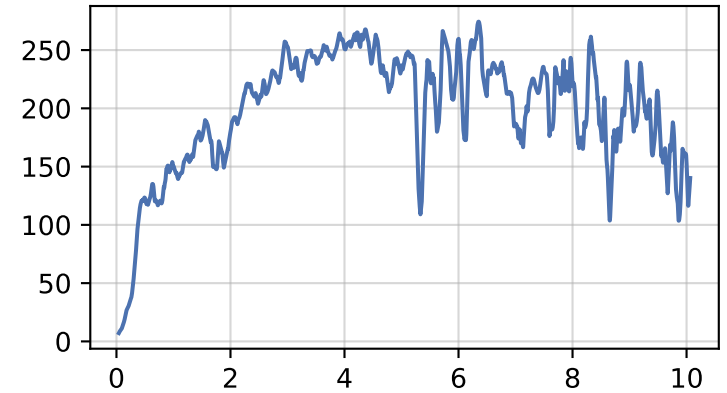
dm_control/cheetah-run-v0
