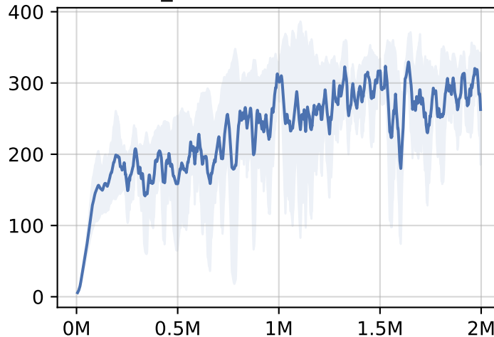
dm_control/walker-walk-v0
