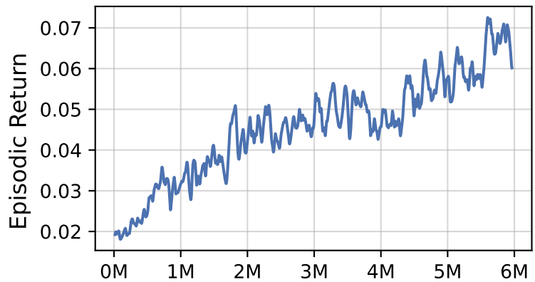
MortarMayhem-Grid-v0
