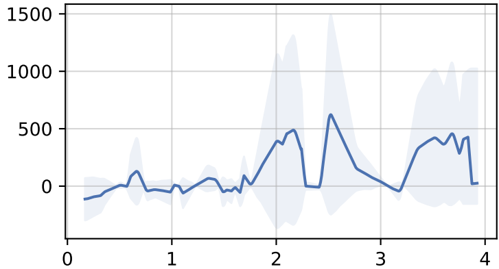
HalfCheetah-v4
