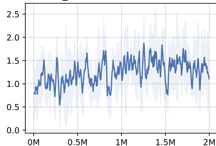
dm_control/walker-run-v0
