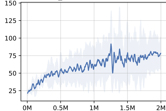
dm_control/walker-run-v0
