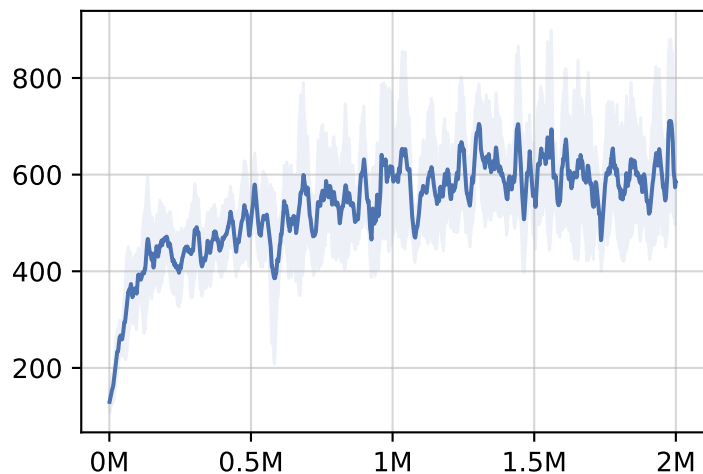
dm_control/humanoid-run-v0
