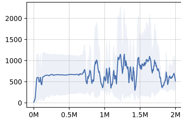
dm_control/humanoid-walk-v0
