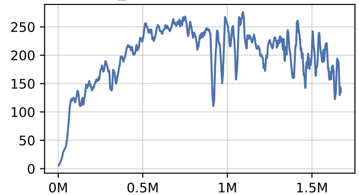
dm_control/cheetah-run-v0
