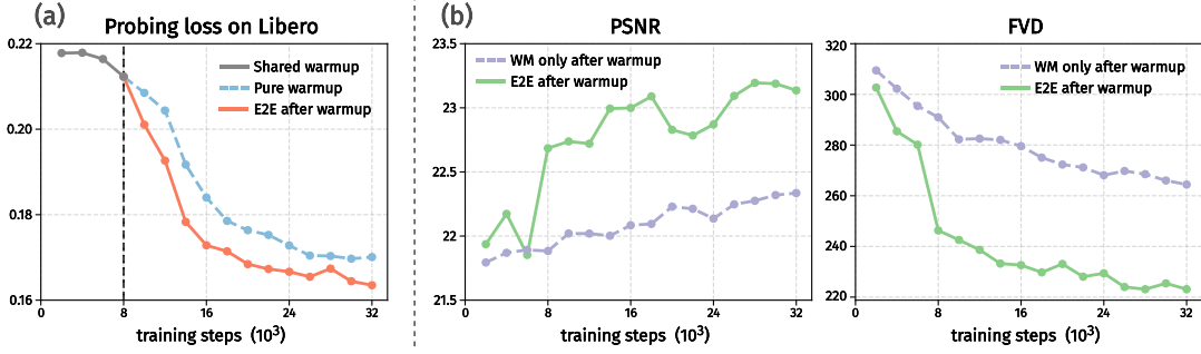
Figure 4: Evidence of synergistic co-evolution. The LAM’s probing loss drops faster when the world model is co-evolving (a), while the world model achieves higher video prediction performance as the LAM improves (b).
