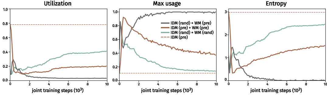
Figure 2: Latent action codebook metrics during joint training of the IDM and world model. “rand” indicates random initialization, while “pre” indicates initialization from pretrained weights. The dashed line shows the codebook metrics of the pretrained IDM. All three subplots share the same legend, shown only in the middle panel for clarity.
