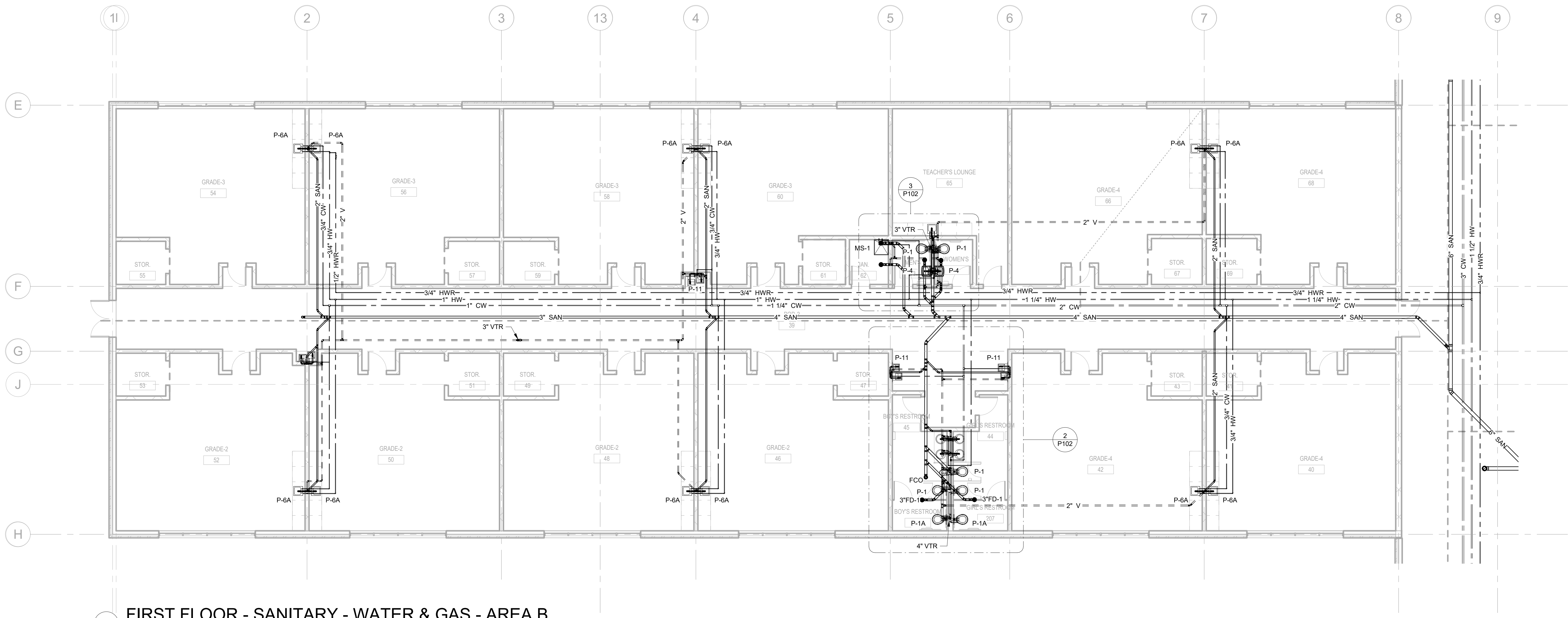
1 FIRST FLOOR - SANITARY - WATER & GAS - AREA B 1/8" = 1'-0"
