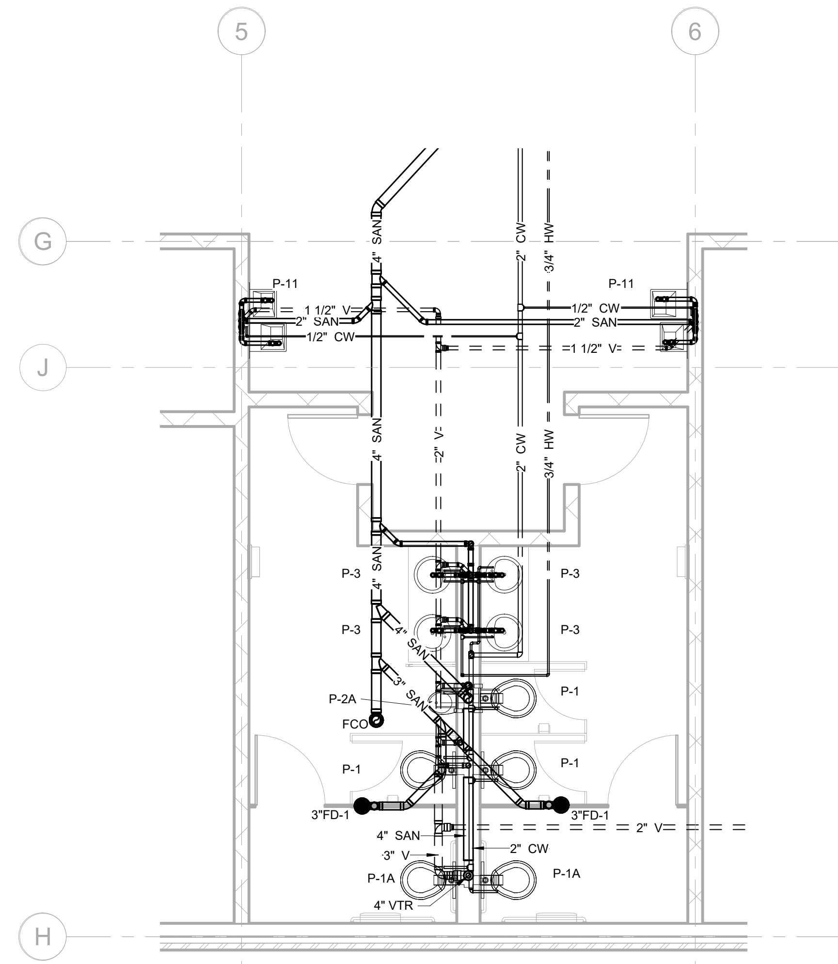
1 FIRST FLOOR - SANITARY - WATER & GAS - AREA B 1/8" = 1'-0"
