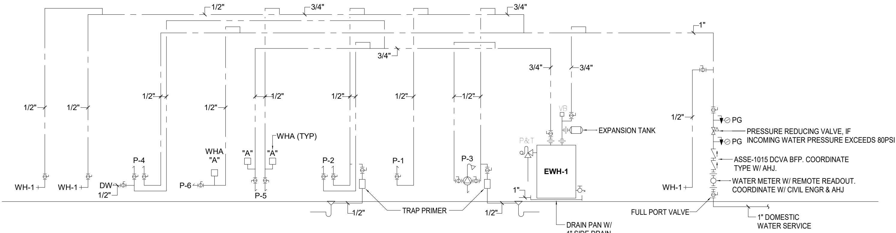
1 WATER RISER DIAGRAM NTS
