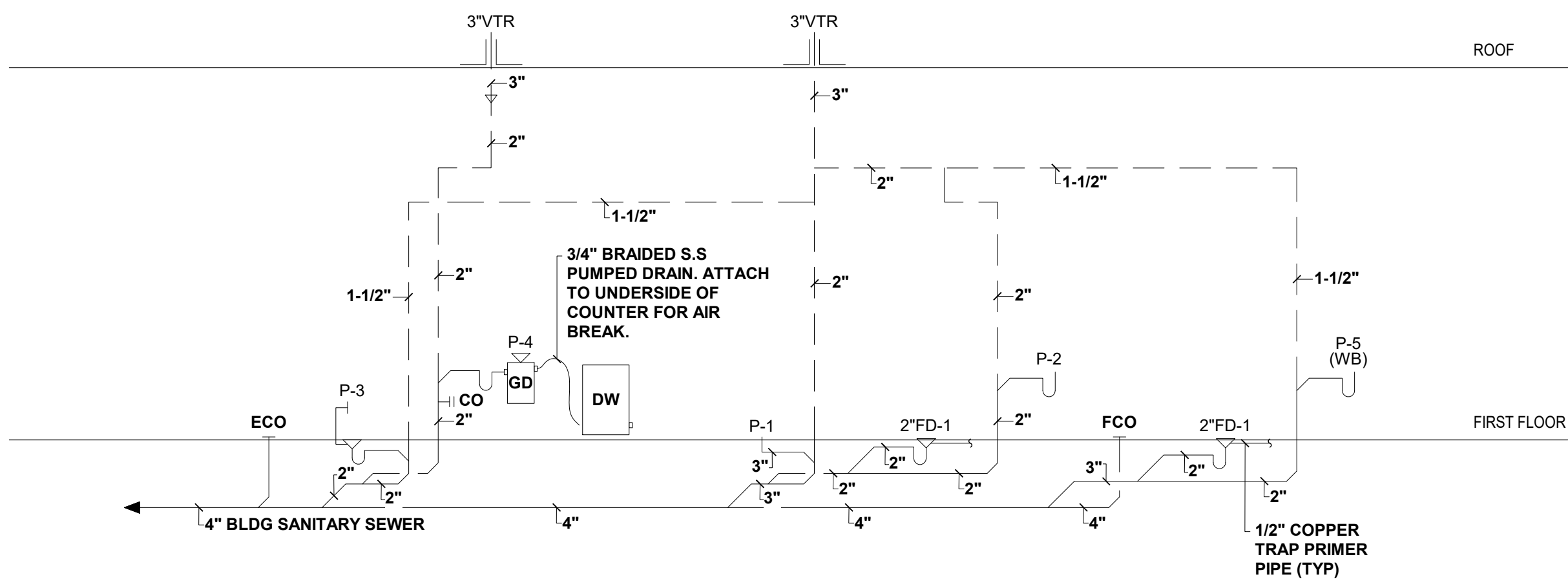
2 SANITARY RISER DIAGRAM NTS
