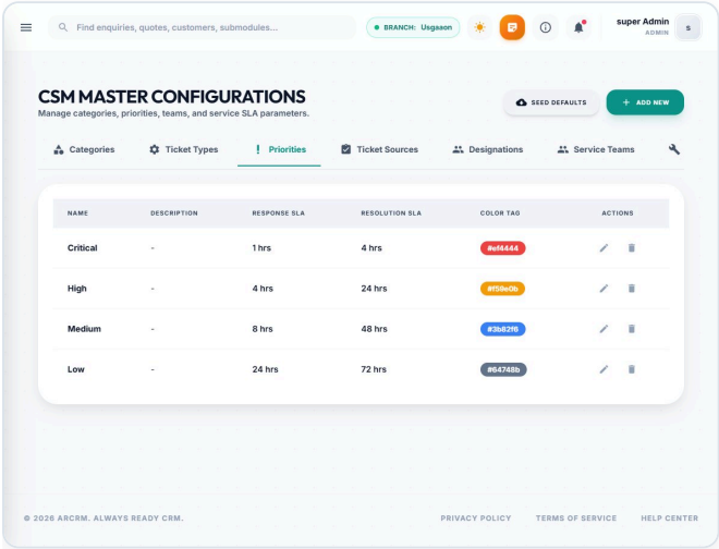
Figure 29. Priorities with their SLA hours.
