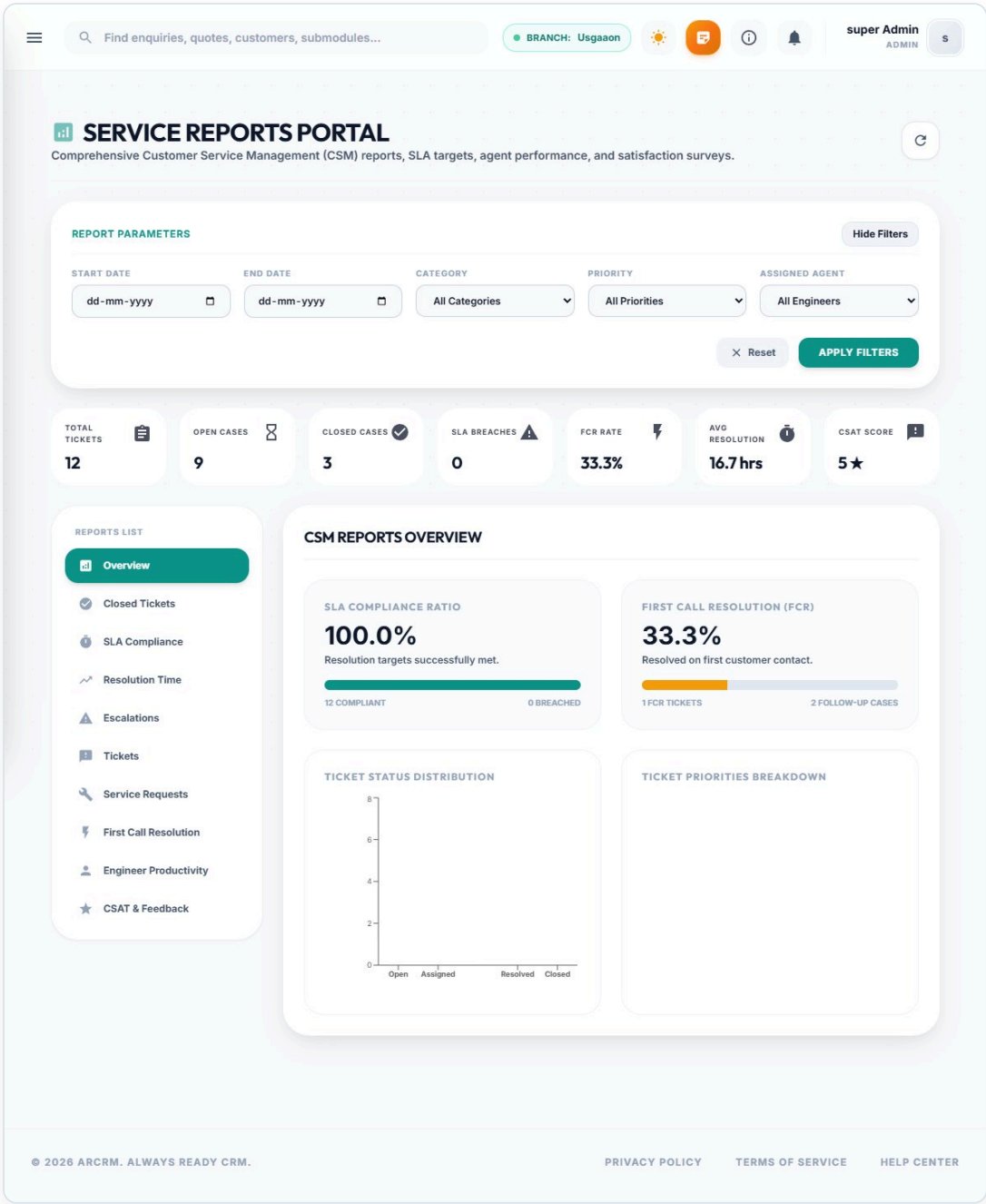
Figure 32. Service Reports Portal: parameters, KPI cards and the Overview report.
