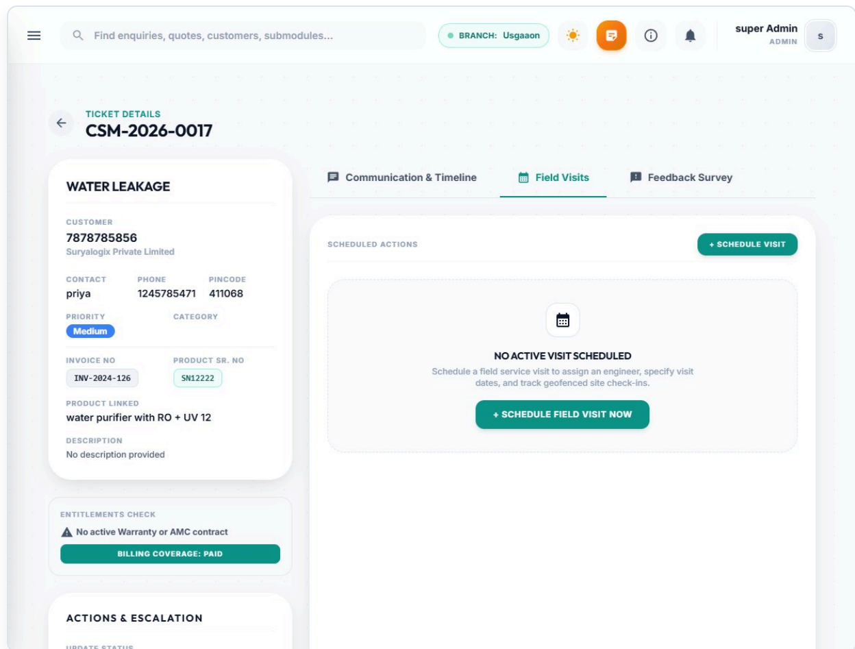
Figure 12. Field Visits tab on a ticket with no active visit.
