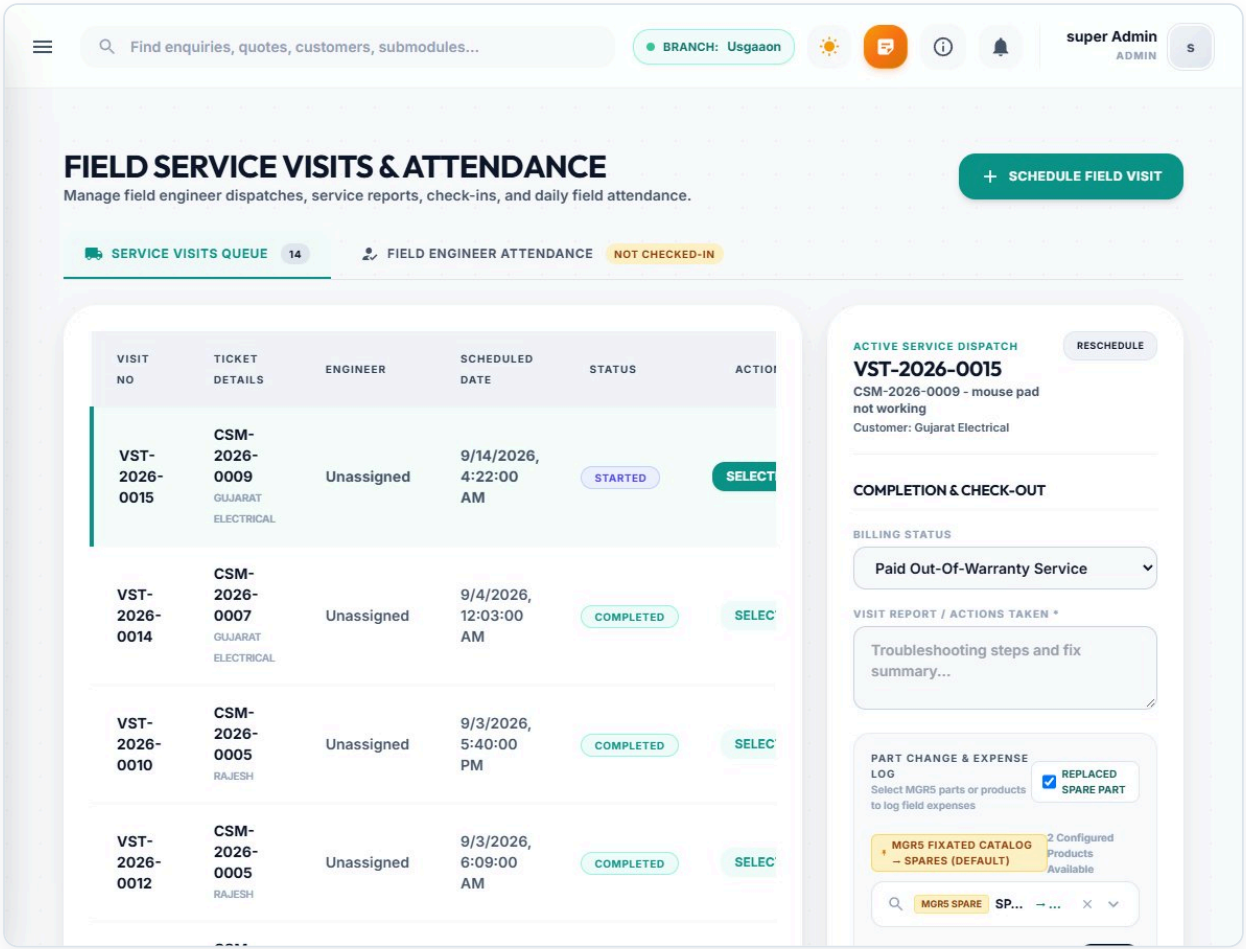
Figure 15. Service Visits Queue with the selected visit's dispatch panel.
