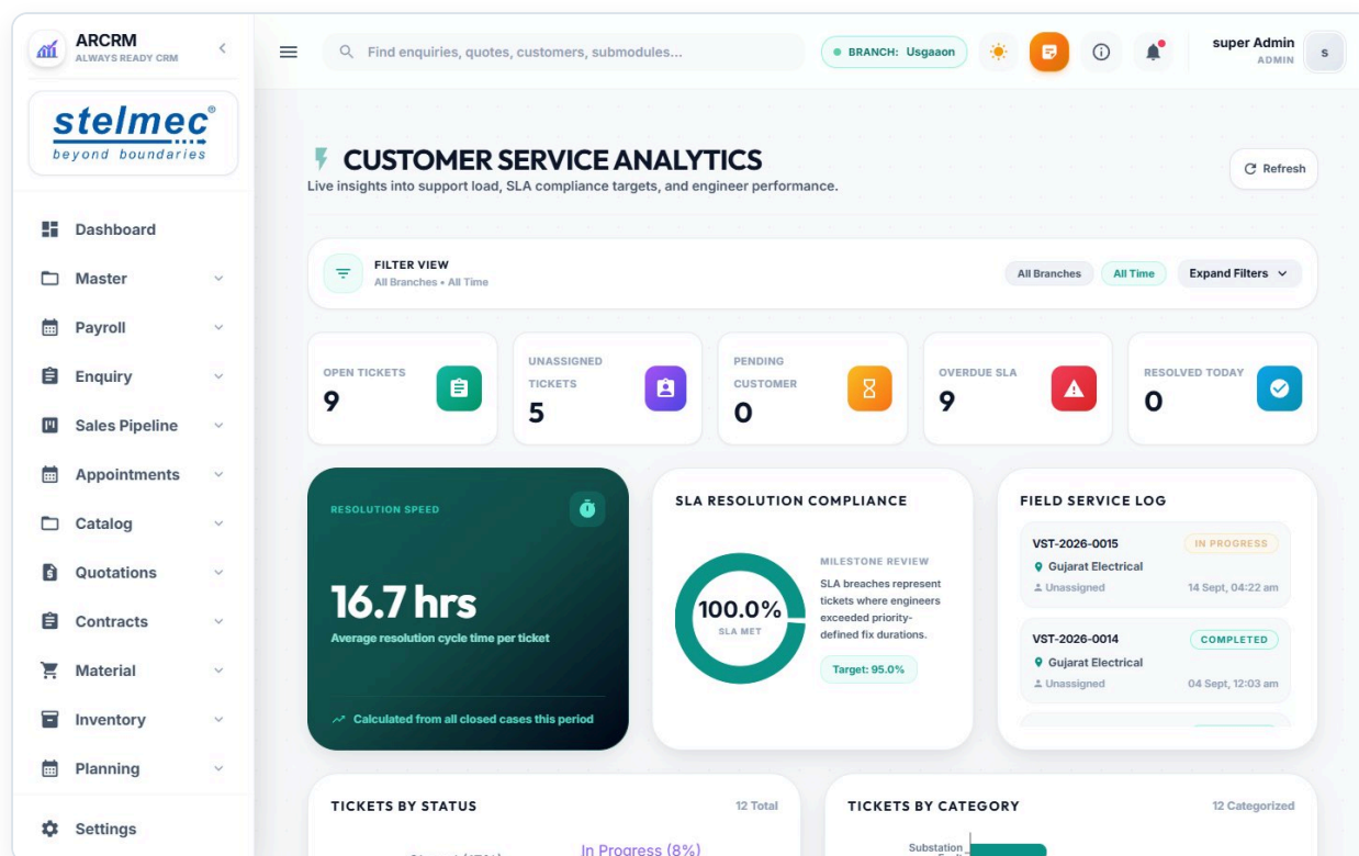
Figure 2. The ARCRM workspace: menu on the left, global search and the branch indicator at the top, and the page content in the centre.
