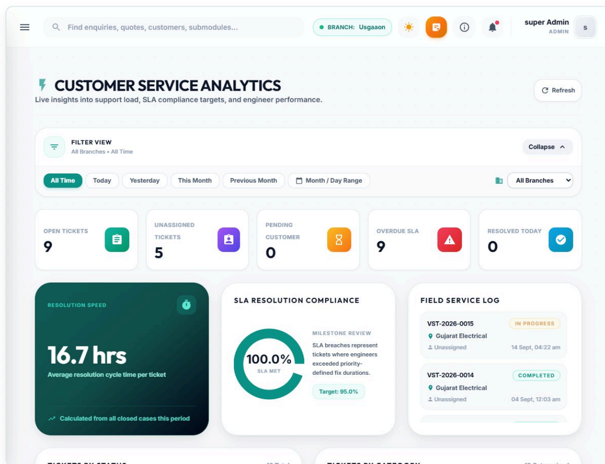
Figure 4. Dashboard filter presets: All Time, Today, Yesterday, This Month, Previous Month, and Month / Day Range.
