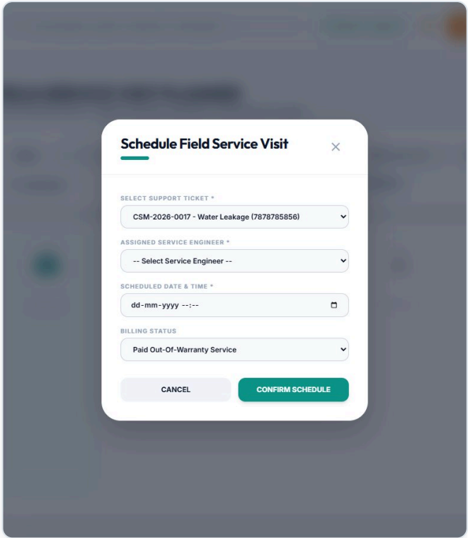
Figure 22. Schedule Field Service Visit from the planner.
