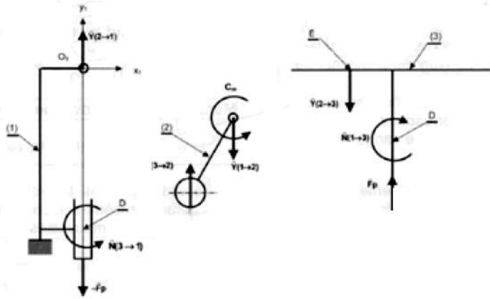
Figure 4 – Actions mécaniques calculables
