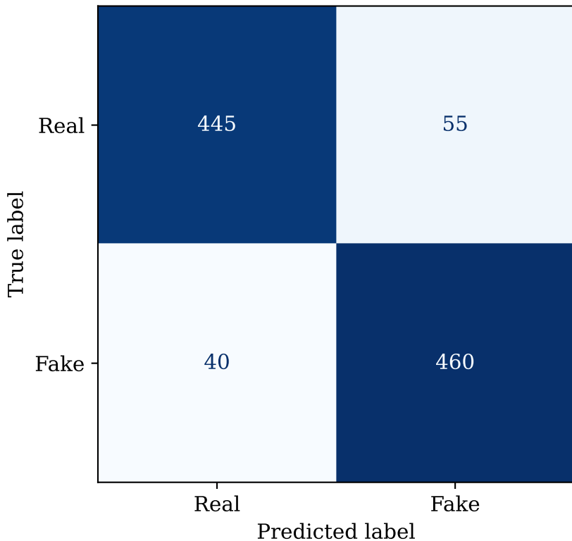
Ensemble Model — Confusion Matrix (Test Set, n=1000)
