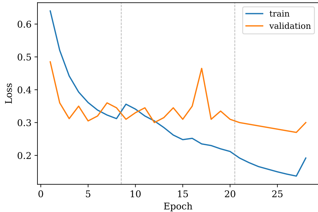
F3Net — Train and Validation Loss
