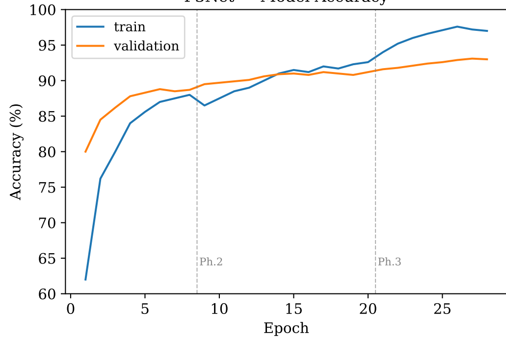
F3Net — Model Accuracy
