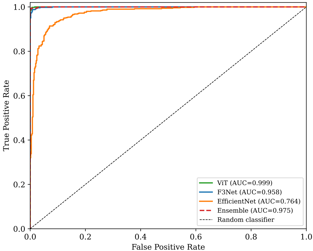
ROC Curves — Per-Model and Ensemble
