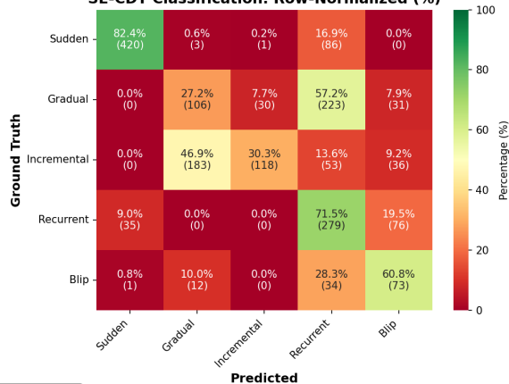
SE-CDT Classification: Row-Normalized (%)
