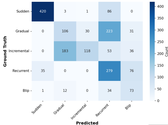
SE-CDT Classification: Counts
