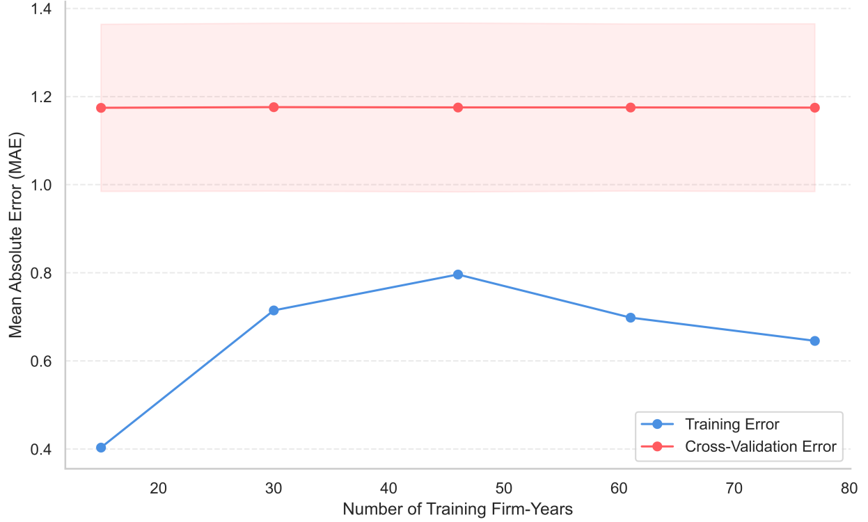
Figure 3: SVR Learning Curve (GroupKFold)
