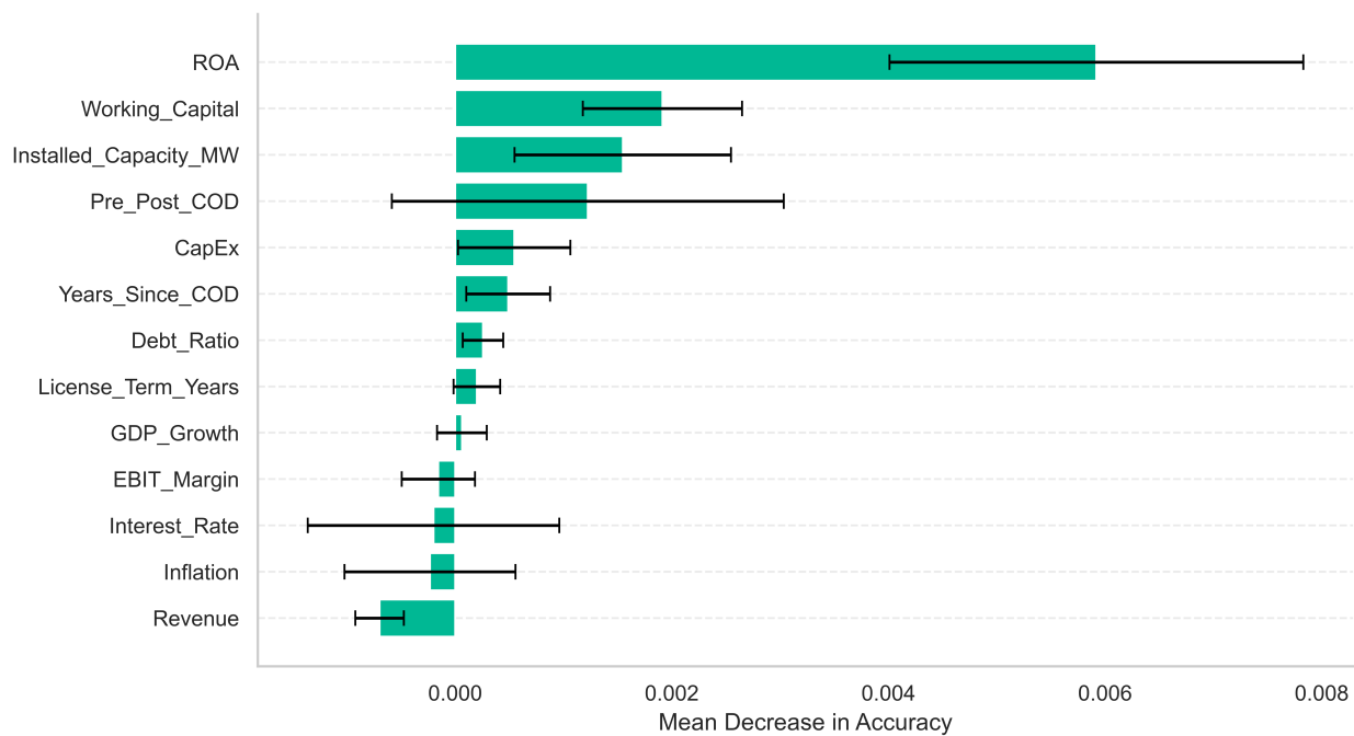
Figure 4: Permutation Importance inside the SVR Kernel ( n = 30, \pm \text{SD} )
