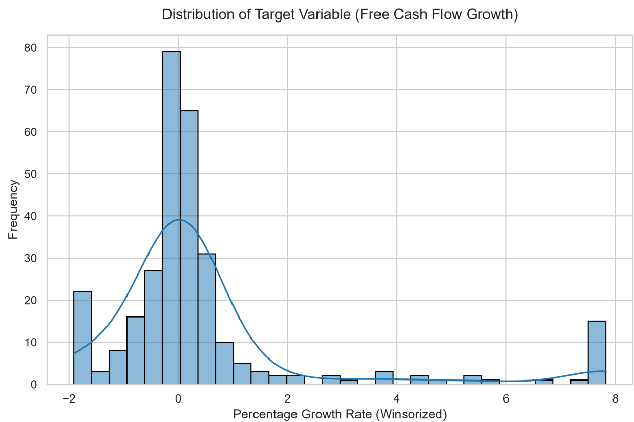
Figure 1: Distribution of Target Variable (Free Cash Flow Growth). Note that the bars at the extreme tails ( \sim -1.8 and \sim 7.5 ) are winsorization artifacts, not organic clusters.
