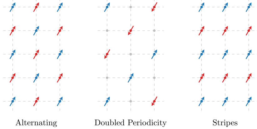
Figure 2.1 Three possible antiferromagnetic structures. Dots and arrows indicate spin abundance on a given site, while empty sites are intended as spin-balanced. Within this text we deal with the lowest-periodicity commensurate phase, the antiferromagnet on left panel.
