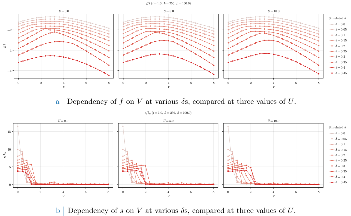
Figure 2.11 | Dependency of free energy (top) and entropy (bottom) densities on V varying the doping \delta and the local repulsion U .
