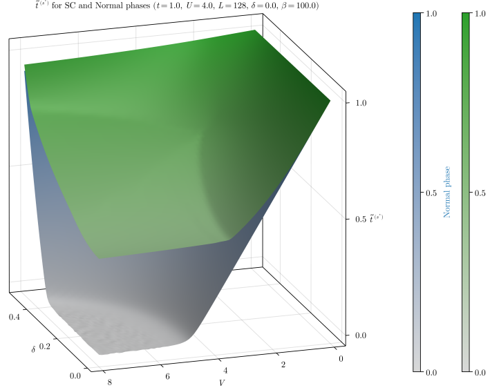
Figure 2.9 | Comparison of the isotropic part of the renormalised hopping \tilde{t}^{(s^*)} for the SC (green) and normal (blue) phases on the (\delta, V) plane. The data from the normal phase are the same of Fig. 1.7.
