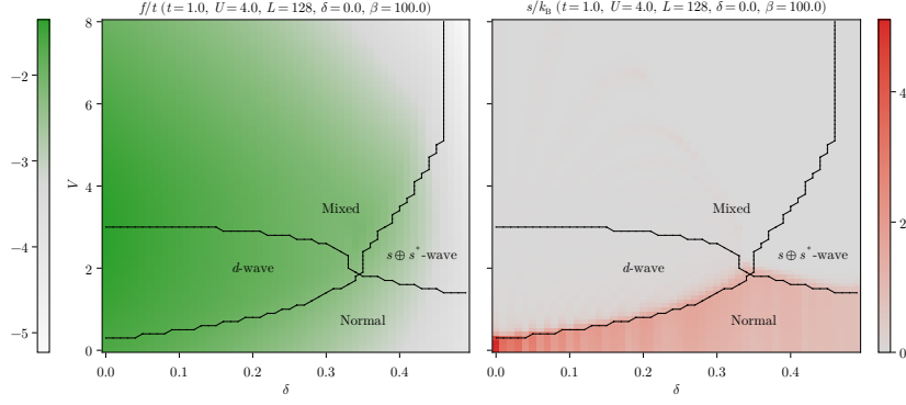
Figure 2.10 | Heatmaps of the free energy and entropy densities at U/t = 4 . The black dotted lines represent the internal boundaries of the singlet SC phase.
