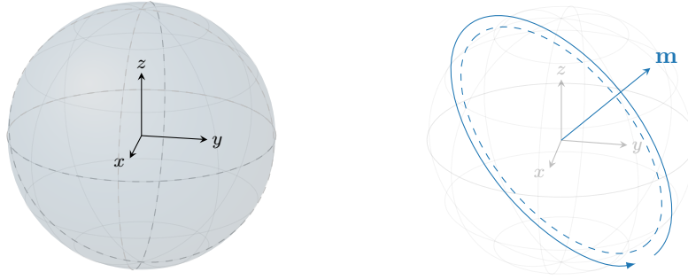
a | SU(2) rotations domain before SSB. b | U(1) rotations domain after SSB.
