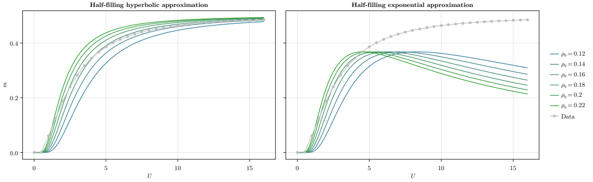
Figure B.3 | Sketch of the analytic expression for m . The left panel shows a family of coloured curves described by Eq. (B.12). The right panel shows a family of coloured curves described by Eq. (B.13), only reasonable at U \rightarrow 0 .
