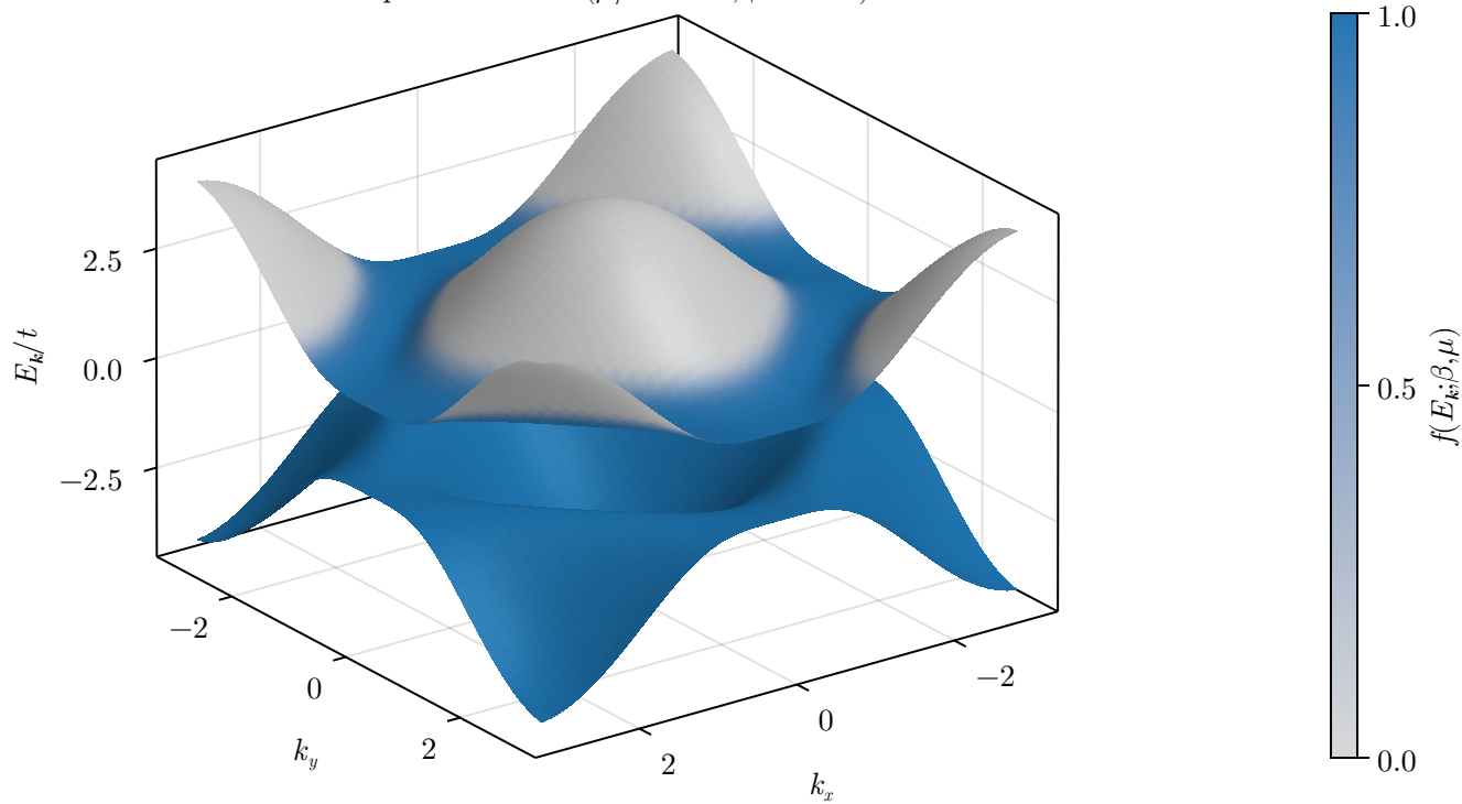
Doped AF bands ( \mu/\Delta = 1.5 , \beta = 10.0 )
