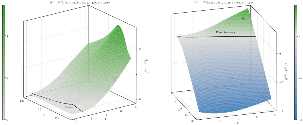
a | Energy difference with normal phase.
