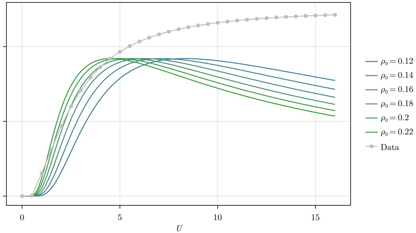
Half-filling exponential approximation
