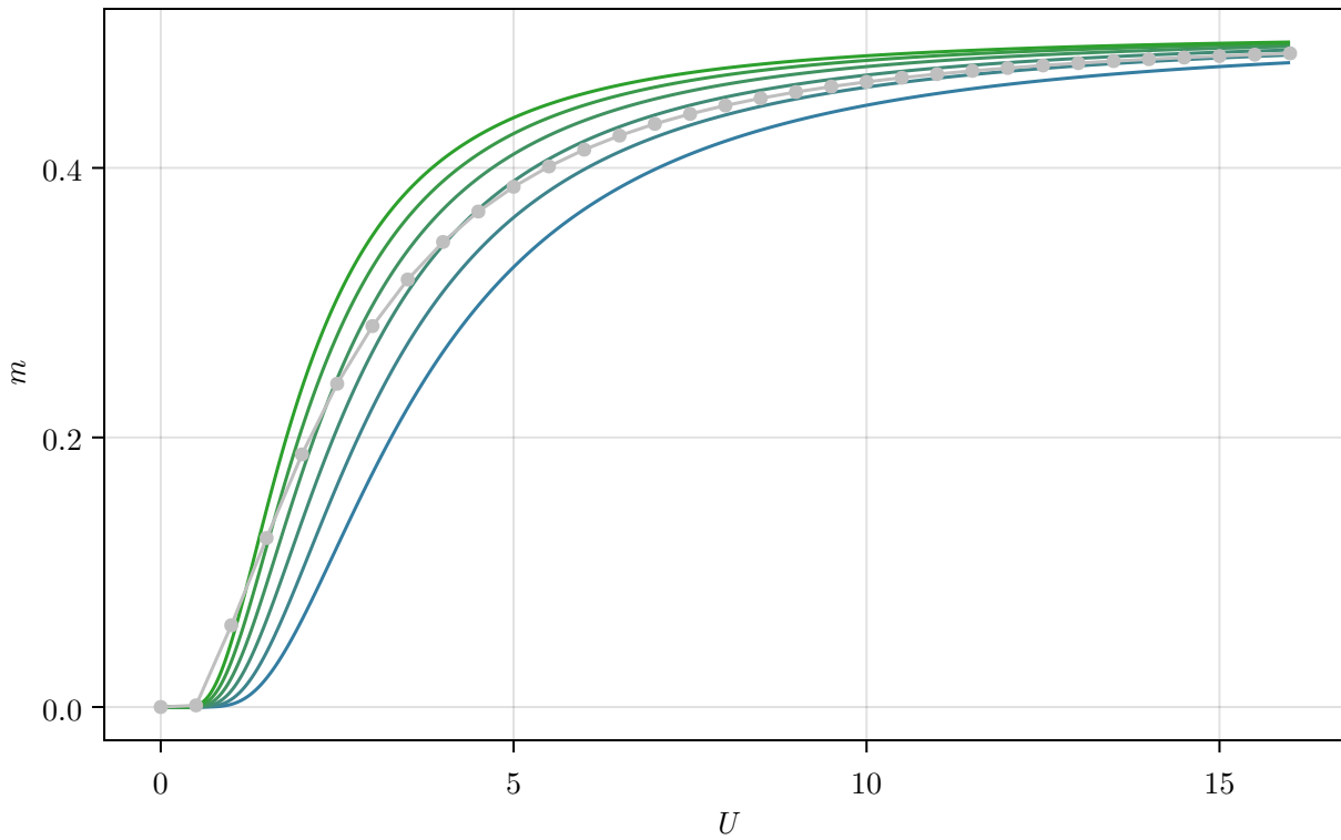
Half-filling hyperbolic approximation
