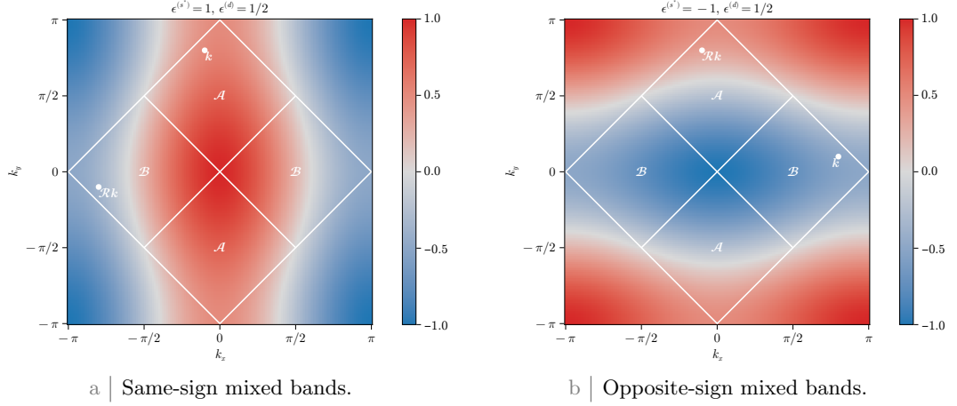
Figure F.3 | Nematic bands \tilde{\epsilon}_{\mathbf{k}} with u^{(s^*)} > 2t/V , u^{(d)} > 0 (top-left) and u^{(s^*)} < 0 , u^{(d)} > 0 (top right). Two example points are reported, connected by a \pi/2 rotation as given in Eqs. (F.10), (F.15)
