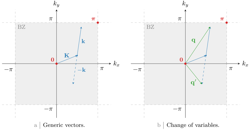
Figure 4.1 | Representation of the variable change used in Eqs. (4.20), (4.21). In Fig. 4.1a generic vectors are considered, for all values of \mathbf{K}, \mathbf{k} \in \text{BZ} . In Fig. 4.1b is depicted the variables change to the new vectors \mathbf{q}, \mathbf{q}' .
