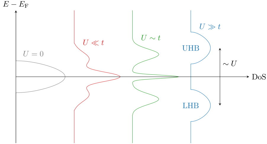
Figure 1.3 | Sketch of the Hubbard DoS as we vary the ratio U/t . For U = 0 (gray plot on the left) we have a free electronic band. As we increase U , two peaks appear while the central coherent peak shrinks. At U \gg t (blue plot on the right), the DoS is separated in upper and lower Hubbard bands (UHB, LHB). E_F is the Fermi energy.
