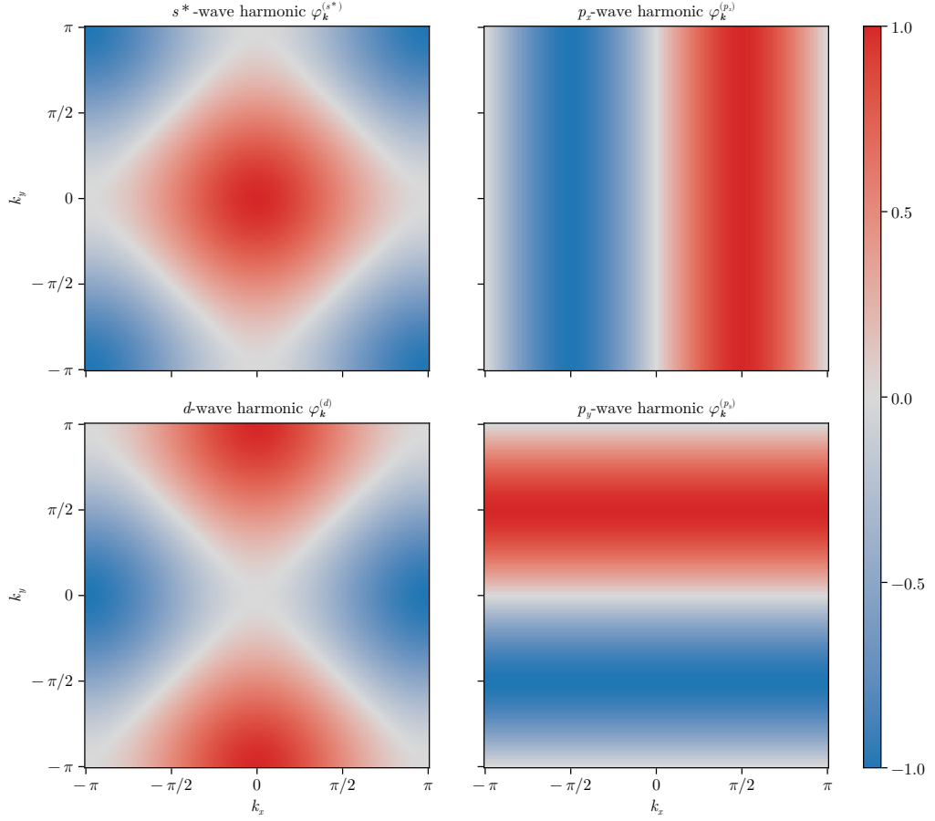
Figure 3.5 | Representation of the harmonics \varphi_{\mathbf{k}}^{(\gamma)} listed in Tab. 3.5 on the BZ. For the s^* and d -wave harmonics, the real part is plotted; for the p_\ell harmonics, the imaginary part is plotted.
