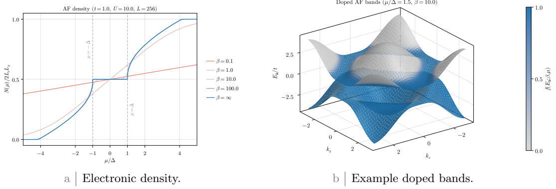
Figure 5.3 | Left panel: electronic density in the AF phase as a function of the chemical potential, computed through Eq. (5.55), at various temperatures. Right panel: example doped bands, with \mu/\Delta = 1.5 set arbitrarily and temperature set to \beta = 10 (absolute units, see Sec. 4.5) to enhance smearing effects around the FS. Single-state filling is proportional to the colour intensity.
