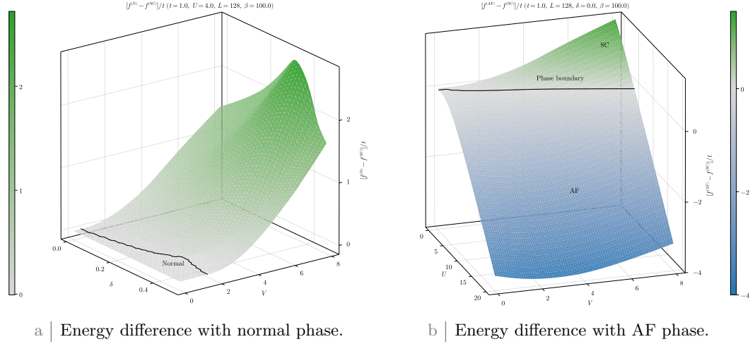
Figure 6.12 | Surface plots of the energies among the three phases. For the normal phase, we use that fact that f^{(SC)} depends weakly on U , while f^{(N)} does not depend on it at all, to limit to the case U/t = 4 . For the AF phase, we limit to the half-filling condition and show data in the (U, V) plane.
