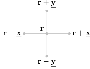
Figure 3.3 | Schematic representation of the four NNs of a given site \mathbf{r} for a planar square lattice.
