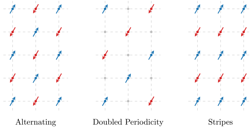
Figure 5.1 | Three possible AF structures. Dots and arrows indicate spin abundance on a given site, while empty sites are intended as spin-balanced. In this thesis, we study the “commensurate” phase, with an alternating AF pattern represented on the left panel.
