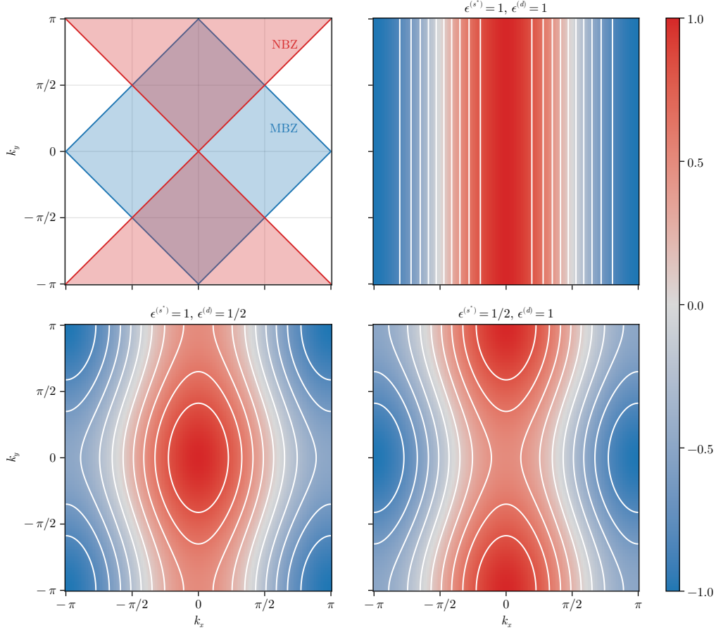
Figure F.1 | Mixed-symmetry bands for the normal phase. The white contours represent level lines. In top-left panel, the MBZ and NBZ are depicted. While these plots only account for positive-defined components, in text is described how to map each one on its counterpart with different sign.
