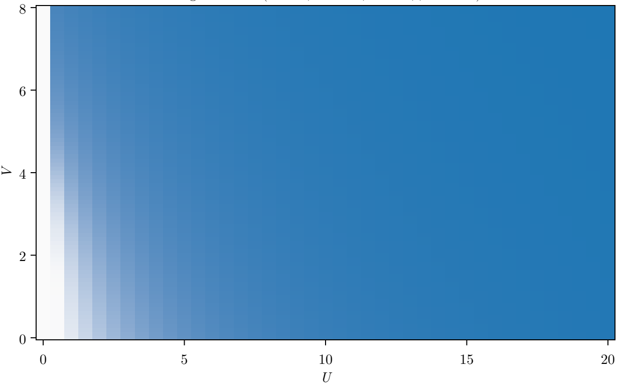
Magnetization ( t = 1.0, L = 128, \delta = 0.0, \beta = 100.0 )
