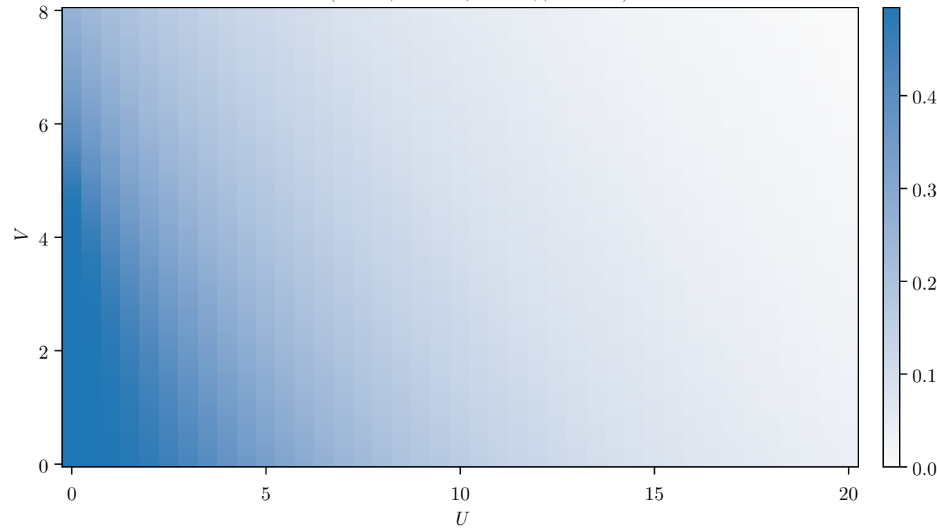
u^{(s^*)} ( t = 1.0, L = 128, \delta = 0.0, \beta = 100.0 )
