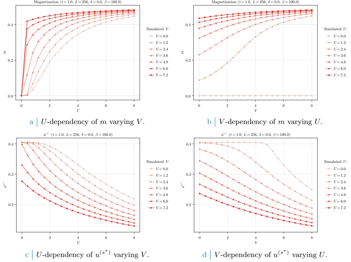
Figure 2.4 | Plot of the self-consistent convergence values for the HFPs m and u^{(s*)} in the AF phase.
