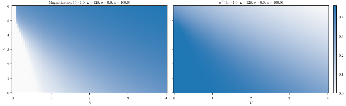
Figure 2.3 | Plot of the self-consistent convergence values for the HFPs m (left panel) and u^{(s*)} (right panel) in the AF phase.
