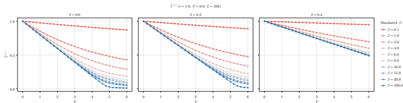
Figure 8: Comparative plots of \tilde{t}^{(s^*)} in the normal phase at various temperatures and dopings.
