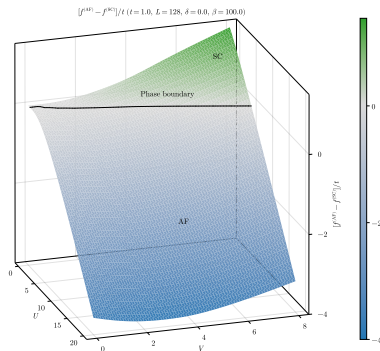
Figure 11: Energy difference: SC versus AF phase.
