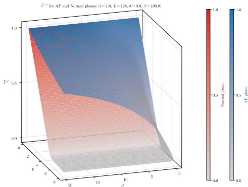
Figure 9: Comparative plot of \tilde{t}^{(s^*)} for normal and AF phase.
