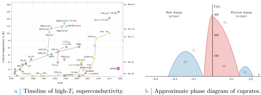
Figure 1.1 | Left: timeline of the discovery of superconductivity in various compounds. The cuprates branch is represented as cyan diamonds. Image source: Refs. [4] and [5], distributed according to the license CC BY-SA 4.0. Right: sketch of the phase diagram of cuprates. These curves result from graphic elaboration and do not refer to any specific physical dataset.
