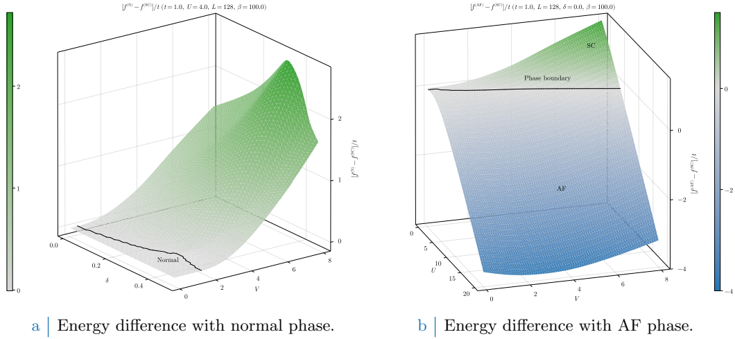
Figure 6.12 | Surface plots of the energies among the three phases. For the normal phase, we use that fact that f^{(\text{SC})} depends weakly on U , while f^{(\text{N})} does not depend on it at all, to limit to the case U/t = 4 . For the AF phase, we limit to the half-filling condition and show data in the (U, V) plane.
