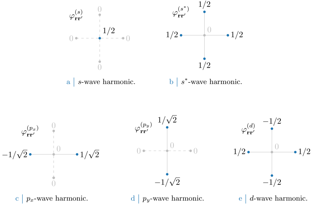
Figure 3.4 | The harmonics listed in Tab. 3.4. In figures, five sites are represented: the hub site \mathbf{r} and its four NNs. Solid lines connect the hub sites to a rim site where the harmonic is non-zero. Dashed lines connect to a rim site where the harmonic is zero.
