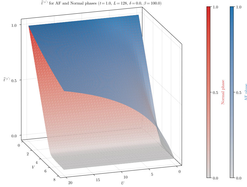
Figure 5.8 | Comparative plot of the converged values for \tilde{t}^{(s*)} for the normal phase and the AF phase.
