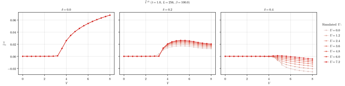
a | Dependency of t^{(d)} on V at various U s, compared at three values of \delta .
