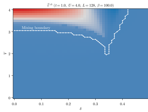
a | Nematic hopping at U = 4 .
