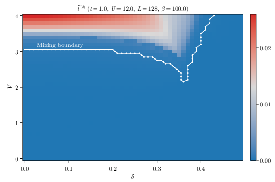
b | Nematic hopping at U = 12 .
