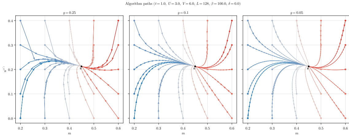
Figure 5.14 | Quiver plot of algorithmic evolution in HFPs space at fixed model parametrization. The black dot \mathbf{v} represents the nonlinear map fixed point, while the colored paths the sequences of HFPs coordinates simulated via iterative HF procedure, starting from different HFPs initialisers (colored dots).
