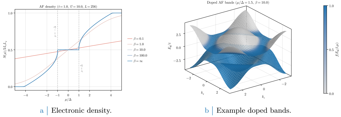
Figure 5.3 Left panel: electronic density in the AF phase as a function of the chemical potential, computed through Eq. (5.53), at various temperatures. Right panel: example doped bands, with \mu/\Delta = 1.5 set arbitrarily and temperature set to \beta = 10 to enhance smearing effects around the FS. Single-state filling is proportional to the colour intensity.
