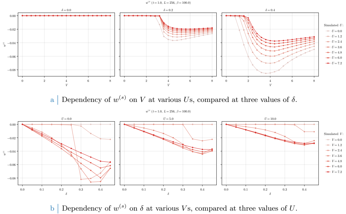
Figure 6.1 | Dependency of the s -wave HFP w^{(s)} on V at fixed U and \delta (top panel, compared figures) and on \delta at fixed V and U (bottom panel, compared figures).
