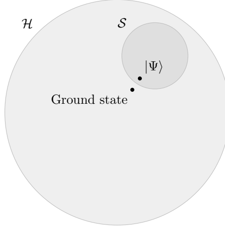
Figure 2.1 | Pictorial representation of the search for the best approximation |\Psi\rangle to the true ground-state inside the subspace S \subset \mathcal{H} .
