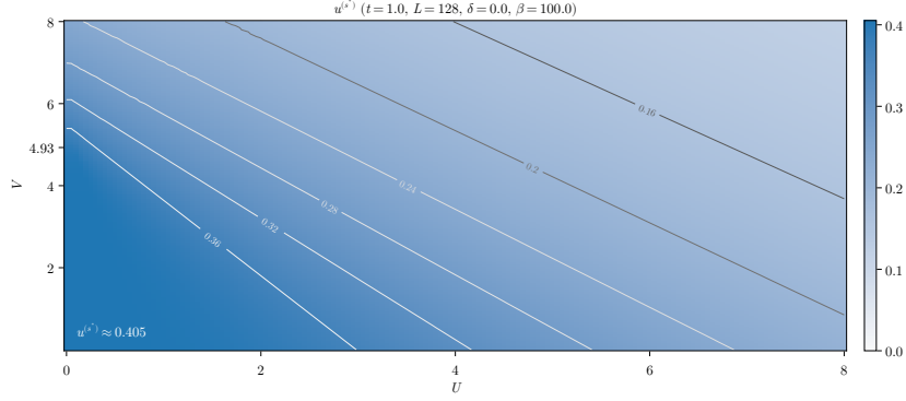
Figure 5.5 | Numerical results for the HFP u^{(s*)} . The gray curves indicate isovalued lines.
