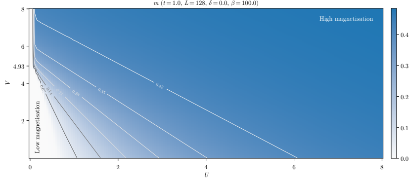
Figure 5.10 | Numerical results for the HFP m . The gray curves indicate isomagnetic lines.
