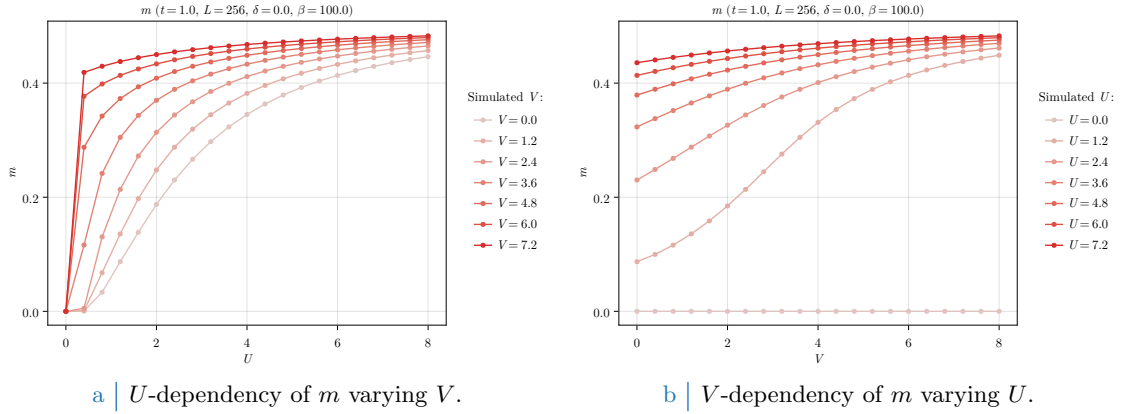
Figure 5.11 | Numerical results for the HFP m as we vary U (left) and V (right), keeping the other variable fixed.
