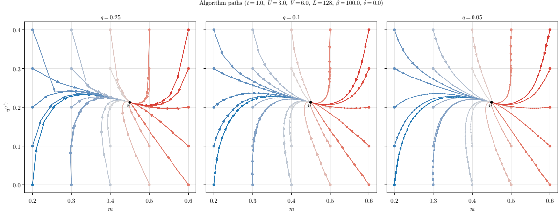
Figure 2.10 | Quiver plot of algorithmic evolution in HFPs space at fixed model parametrization. The black dot \mathbf{v} represents the nonlinear map fixed point, while the colored paths the sequences of HFPs coordinates simulated via iterative HF procedure, starting from different HFPs initializers (colored dots).
