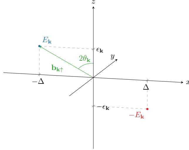
Figure 3.1 | Pseudo-magnetic field originating from mean-field treatment of the square Hubbard hamiltonian. Here, only the \sigma = \uparrow situation is plotted.
