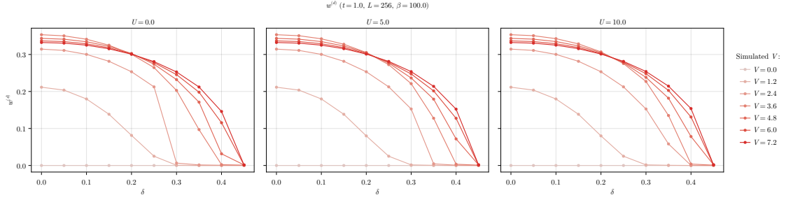
b | Dependency of w^{(d)} on \delta at various V s, compared at three values of U .
