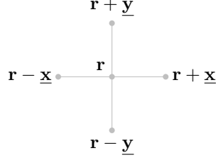
Figure 2.2 | Schematic representation of the four NNs of a given site i for a planar square lattice.
