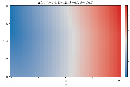
Figure 3.11 | Difference of free energies for the normal phase minus the AF phase.
