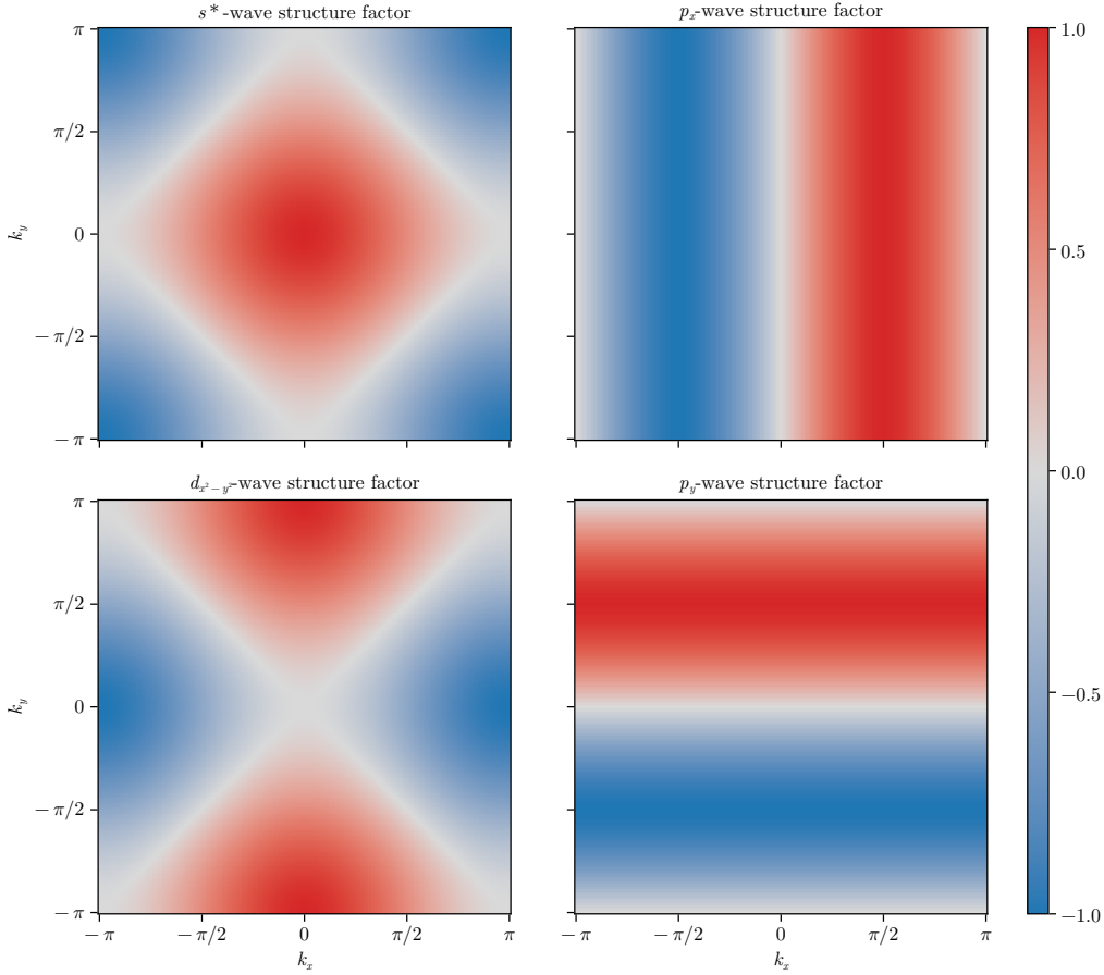
Figure 1.5 | Representation of the various structure factors listed in Tab. 1.5 on the BZ. For the s^* and d_{x^2-y^2} -wave factors, the real part is plotted; for the p_\ell factors, the imaginary part is plotted.
