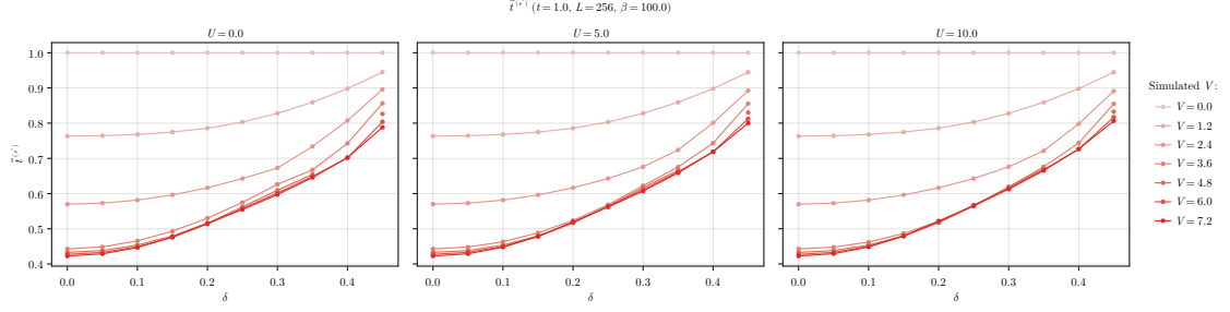
b | Dependency of t^{(s)} on \delta at various V s, compared at three values of U .
