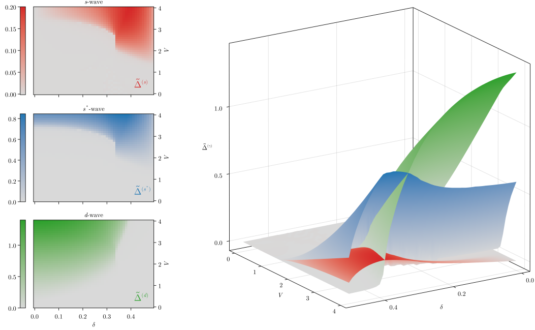
Figure 1.4 | Plot of the singlet gap harmonics \tilde{\Delta}_k^{(\gamma)} , with \gamma = s, s^*, d at U = 4 . The panels on the left show the three harmonics separately as heatmaps, while the surface plot on the right shows them comparatively.
