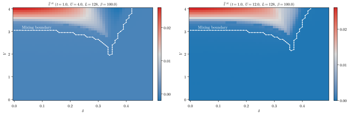
a | Nematic hopping at U = 4 .
