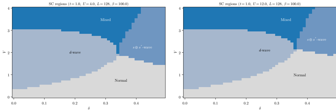
a | SC regions at U = 4 .
