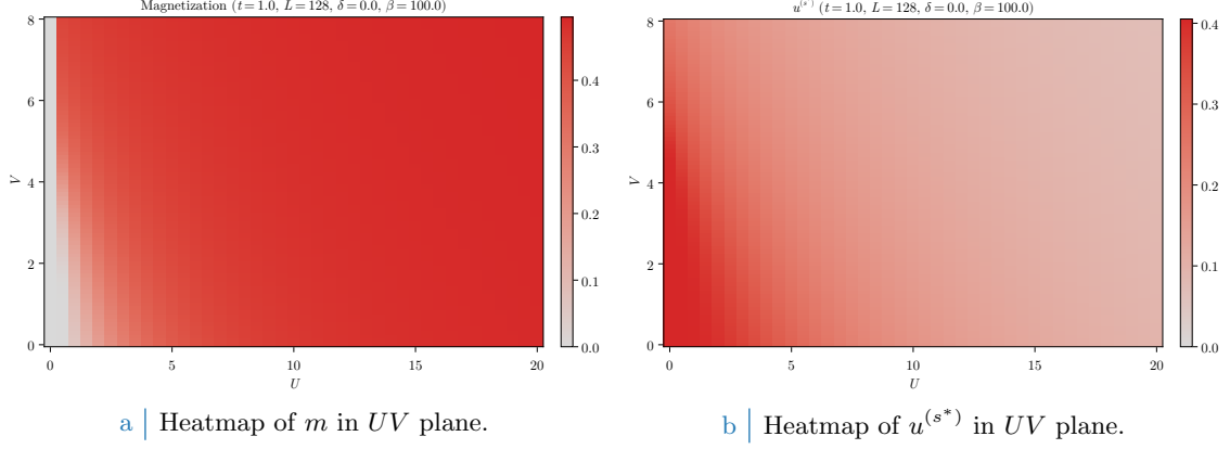
Figure 2.3 | Plot of the self-consistent convergence values for the HFPs m and u^{(s*)} in the AF phase.
