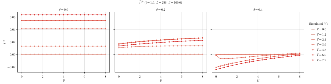
a | U dependency of t^{(d)} at various \delta s.
