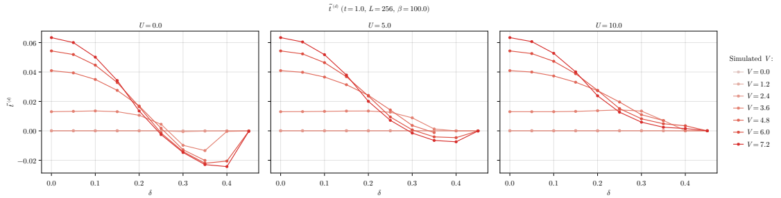
b | \delta dependency of t^{(d)} at various U s.
