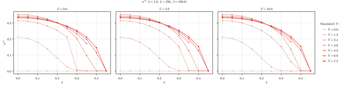
b | \delta dependency of w^{(d)} at various U s.
