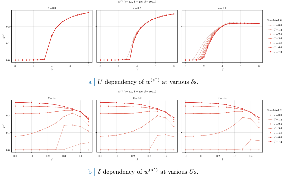
Figure 1.2 | Dependency of the s -wave gap varying the doping \delta and the local repulsion U . In the top panel we compare three doping levels \delta = 0.0, 0.2, 0.4 varying 0 \leq U \leq 8 . In the bottom panel we compare three repulsion values U = 0.0, 5.0, 10.0 varying 0 \leq \delta \leq 0.45 .
