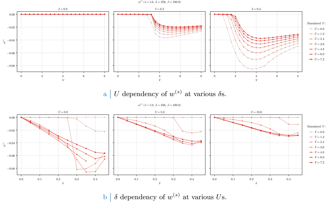
Figure 1.1 | Dependency of the s -wave gap varying the doping \delta and the local repulsion U . In the top panel we compare three doping levels \delta = 0.0, 0.2, 0.4 varying 0 \leq U \leq 8 . In the bottom panel we compare three repulsion values U = 0.0, 5.0, 10.0 varying 0 \leq \delta \leq 0.45 .
