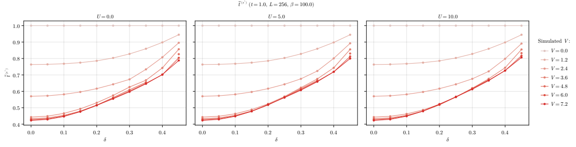
b | \delta dependency of t^{(s*)} at various U s.
