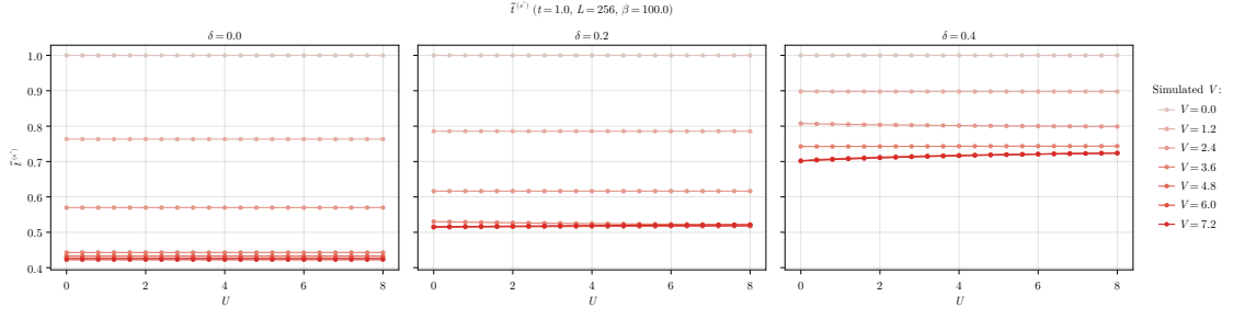
a | U dependency of t^{(s*)} at various \delta s.
