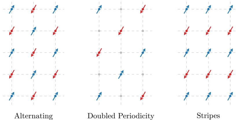
Figure 5.1 | Three possible antiferromagnetic structures. Dots and arrows indicate spin abundance on a given site, while empty sites are intended as spin-balanced. Within this text we deal with the lowest-periodicity commensurate phase, the antiferromagnet on left panel.
