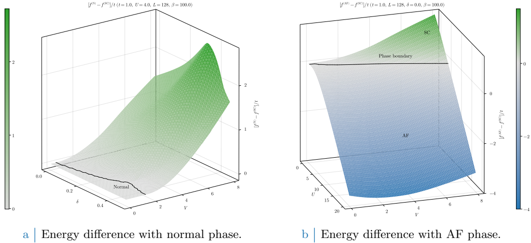
Figure 6.12 | Surface plots of the energies among the three phases. For the normal phase, we use that fact that f^{(\text{SC})} depends weakly on U , while f^{(\text{N})} does not depend on it at all, to limit to the case U/t = 4 . For the AF phase, we limit to the half-filling condition and show data in the (U, V) plane.
