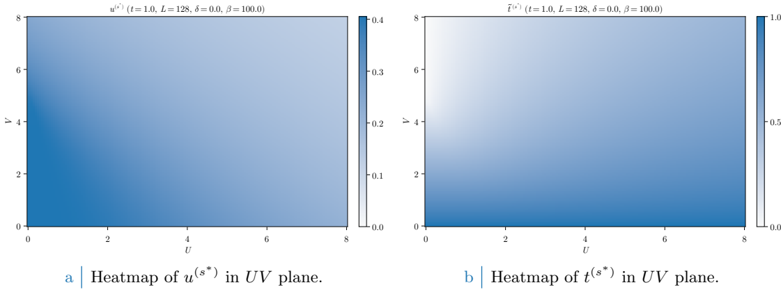
Figure 2.8 | Data for the HFP u^{(s*)} and \tilde{t}^{(s*)} varying both U and V .
