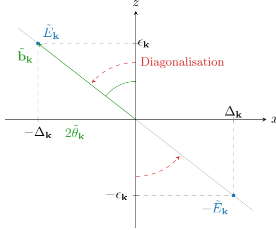
Figure 2.2 | Sketch of the diagonalisation procedure for the HM antiferromagnet. To diagonalise the HF hamiltonian, we align the z axis with the pseudo-field.
