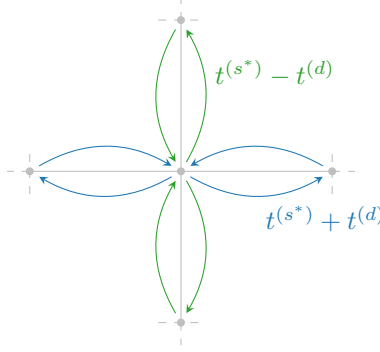
Figure 1.2 | Graphic rendition of anisotropic hopping, with a s^* -wave component (symmetric by \pi/2 rotations) and a d -wave component (antisymmetric).
