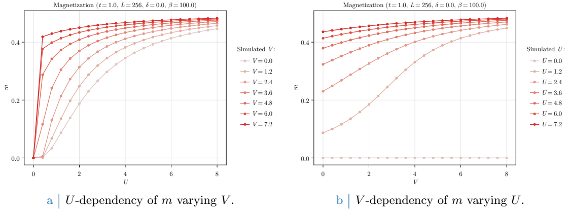
Figure 2.4 | Plot of the self-consistent convergence values for the HFPs m and u^{(s^*)} in the AF phase.
