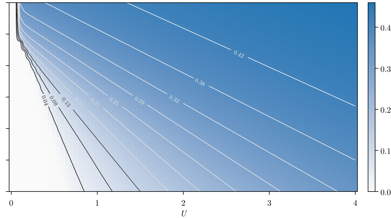
Magnetization ( t = 1.0 , L = 128 , \delta = 0.0 , \beta = 100.0 )
