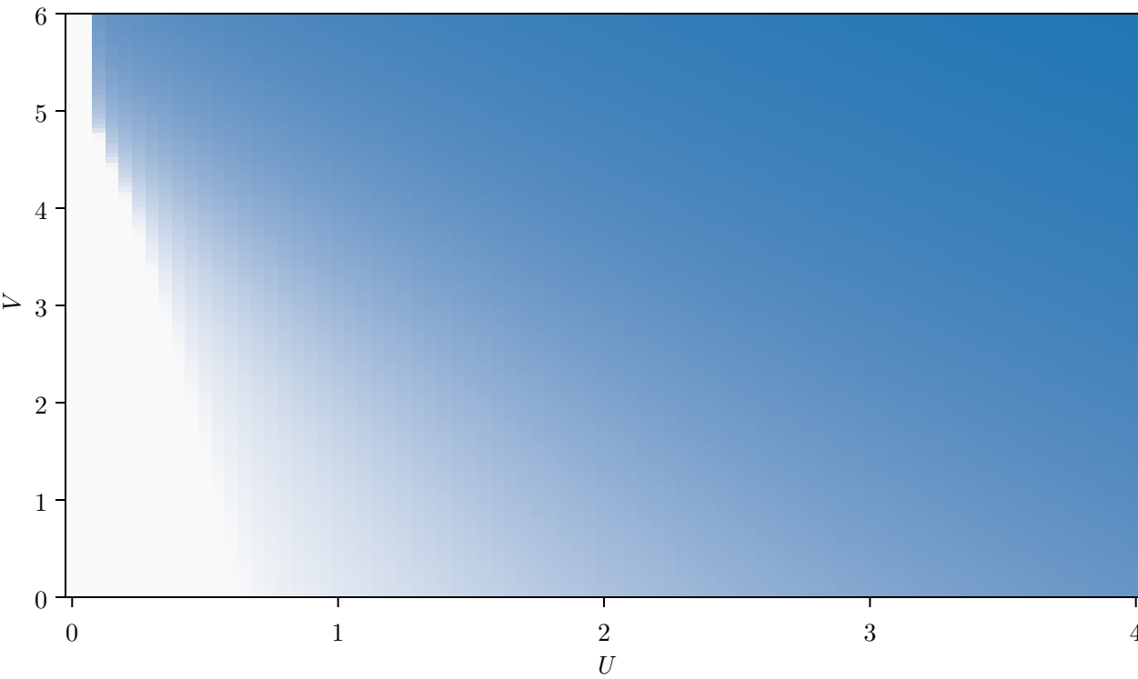
Magnetization ( t = 1.0 , L = 128 , \delta = 0.0 , \beta = 100.0 )
