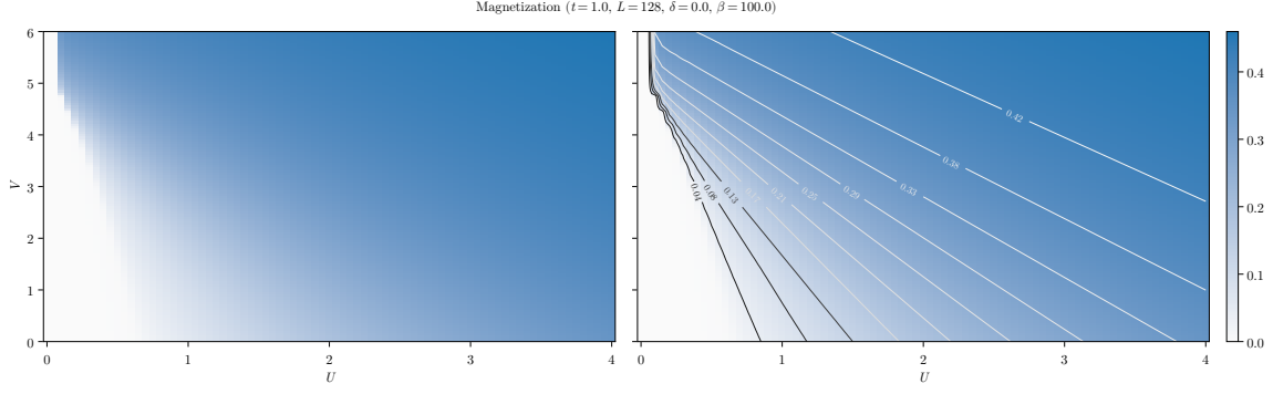
Figure 2.3 | Plot of the self-consistent convergence values for m (left panel) and isomagnetic curves computed on the same data (right panel). The solid lines in the right panel represent those paths in parametric space along which magnetization is constant. [Are U = 0.05 data correct?]
