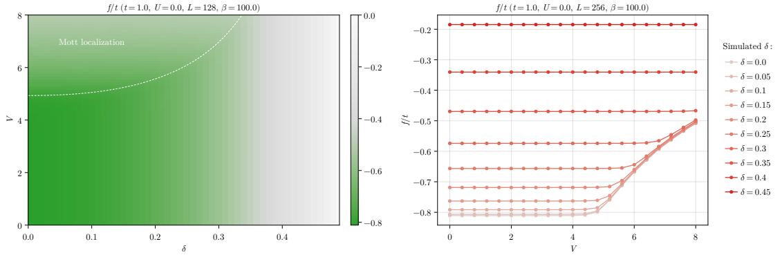
a | Heatmap of f in \delta V plane.
