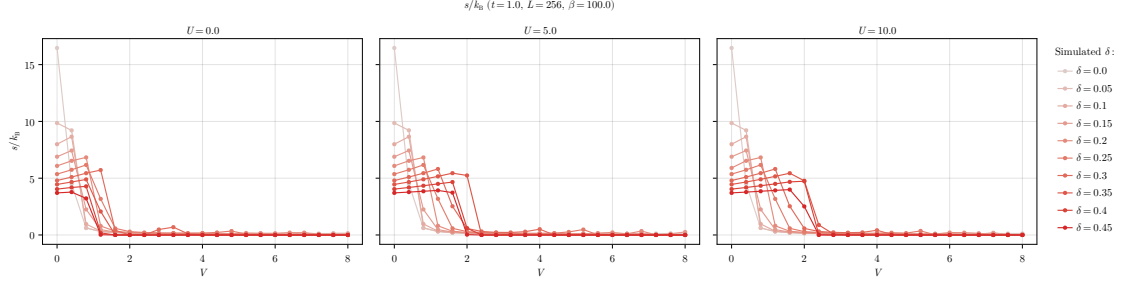
b | Dependency of s on V at various \delta s, compared at three values of U .
