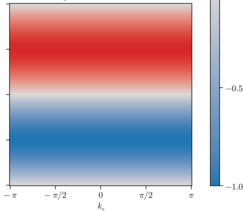
p_y -wave harmonic \varphi_{\mathbf{k}}^{(p_y)}
