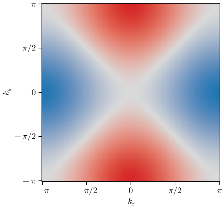
d -wave harmonic \varphi_{\mathbf{k}}^{(d)}
