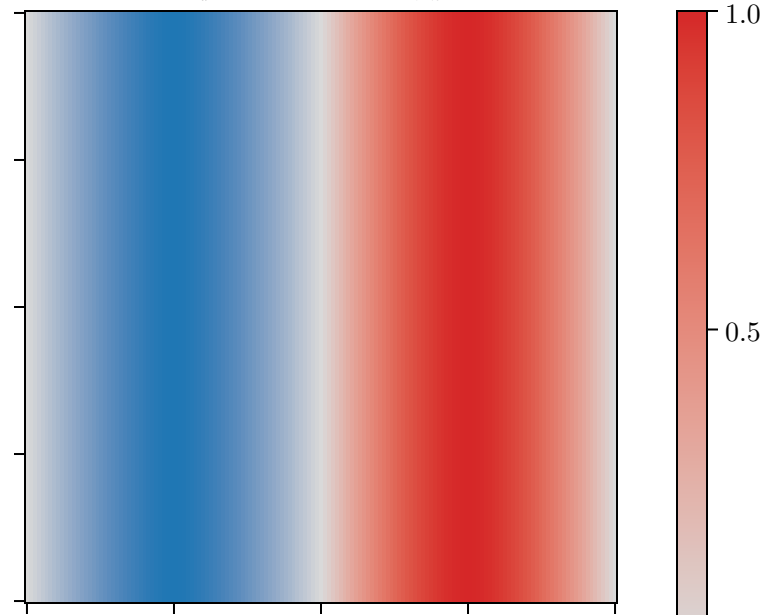
p_y -wave harmonic \varphi_{\mathbf{k}}^{(p_y)}
