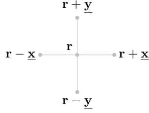
Figure 3.3 | Schematic representation of the four NNs of a given site \mathbf{r} for a planar square lattice.
