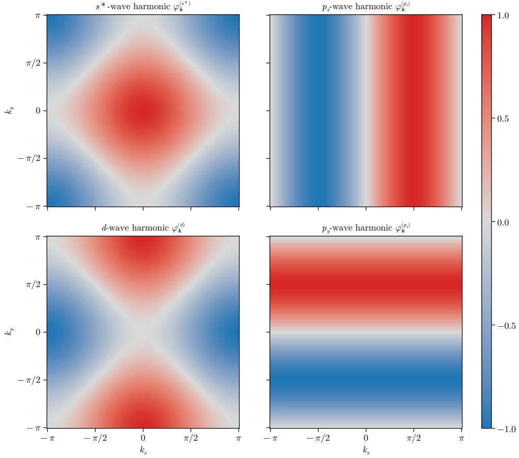
Figure 3.5 | Representation of the harmonics \varphi_{\mathbf{k}}^{(\gamma)} listed in Tab. 3.5 on the BZ. For the s^* and d -wave harmonics, the real part is plotted; for the p_\ell harmonics, the imaginary part is plotted.
