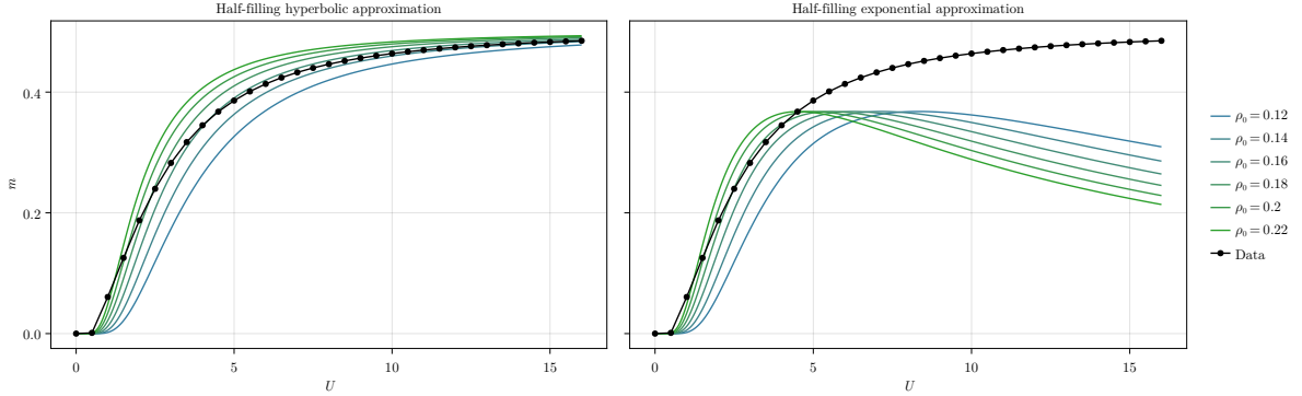
Figure D.3 | Sketch of the analytic expression for m , compared with the numerical results (black dots). The left panel shows a family of coloured curves described by Eq. (D.12). The right panel shows a family of coloured curves described by Eq. (D.13), which approximates m only at U \rightarrow 0 .
