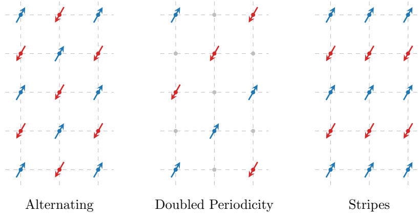
Figure 5.1 | Three possible AF structures. Dots and arrows indicate spin abundance on a given site, while empty sites are intended as spin-balanced. In this thesis, we study the “commensurate” phase, with an alternating AF pattern represented on the left panel.
