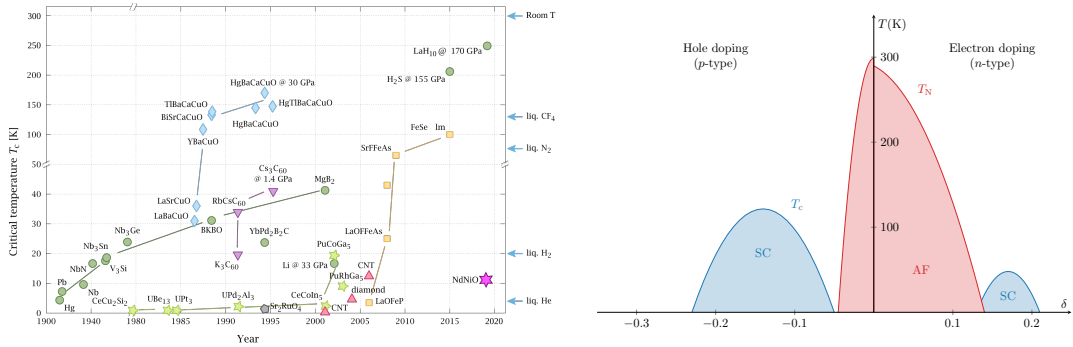
a | Timeline of high- T_c superconductivity.
