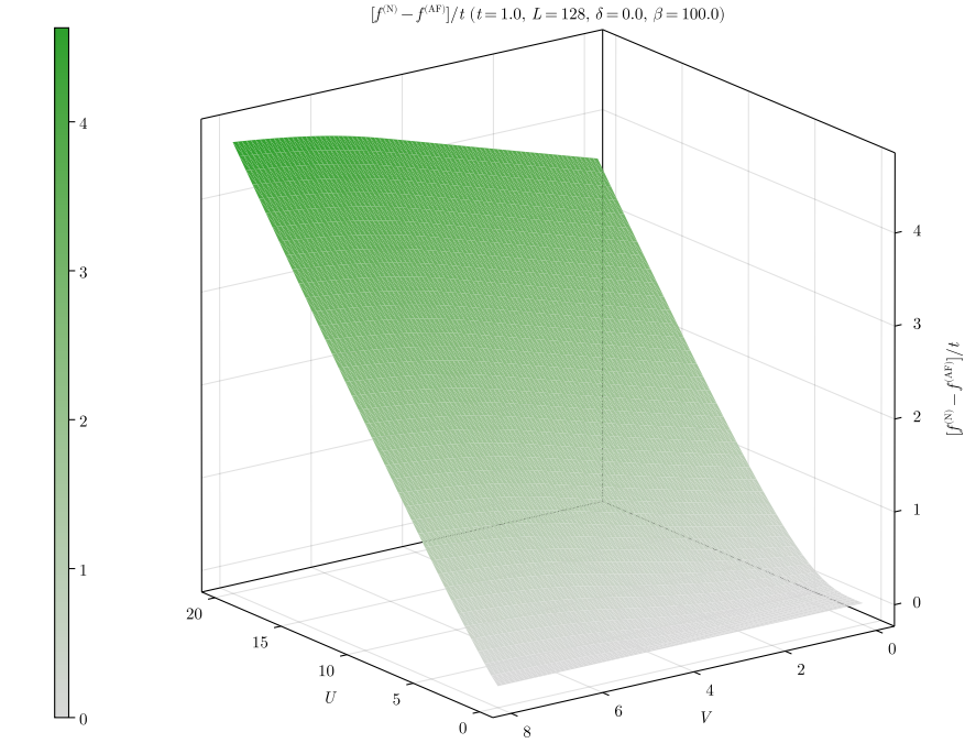
Figure 5.12 | Difference of free energies for the normal phase and the AF phase.
