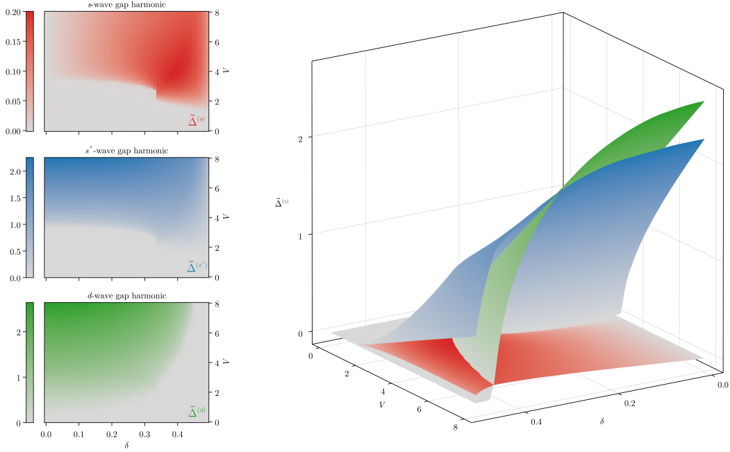
Figure 6.4 | Plot of the singlet gap harmonics \tilde{\Delta}^{(\gamma)} , with \gamma = s, s^*, d at U/t = 4 . The panels on the left show the three harmonics separately as heatmaps, while the surface plot on the right shows them comparatively.
