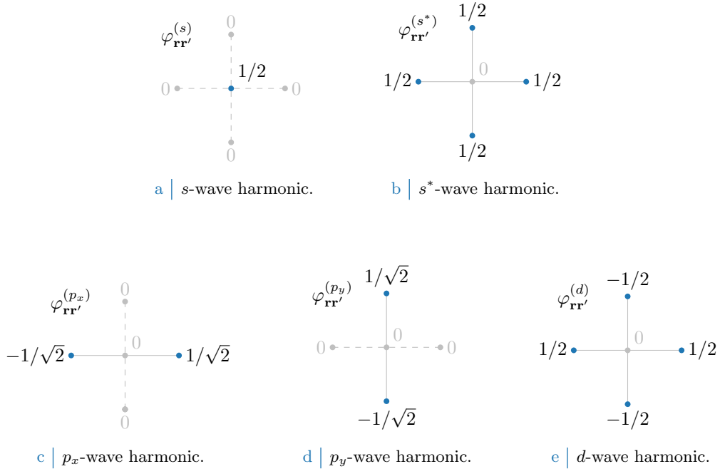
Figure 3.4 | The harmonics listed in Tab. 3.4. In figures five sites are represented: the hub site \mathbf{r} and its four NNs. Solid lines connect the hub sites to a rim site where the harmonic is non-zero. Dashed lines connect to a rim site where the harmonic is zero.
