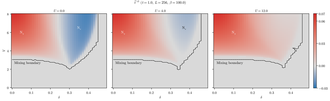
Figure 6.7 Heatmap of the anisotropic component of renormalised hopping, \tilde{t}^{(d)} , at U/t = 0, 4, 12 from left to right. The dataset is the same of Fig. 6.5, and the mixing boundary is the set of points separating the mixed region from the rest of the phases.
