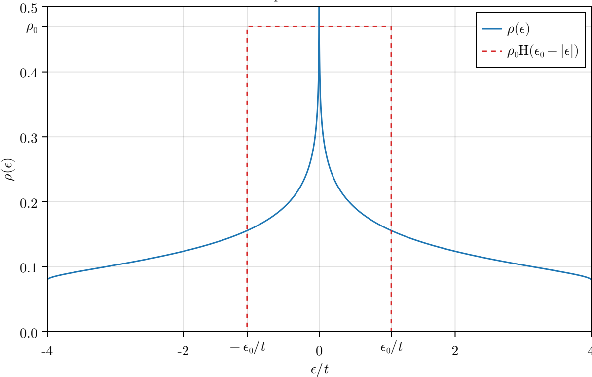
Square lattice DoS
