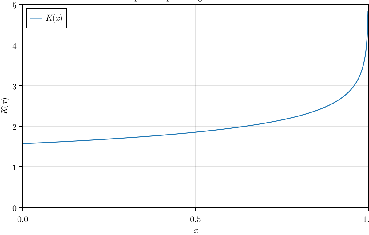
Complete elliptic integral of the first kind
