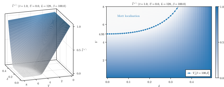
Figure 8: Numerical results for \tilde{t}^{(s^*)} and critical Mott boundary (dotted line in the right plot).
