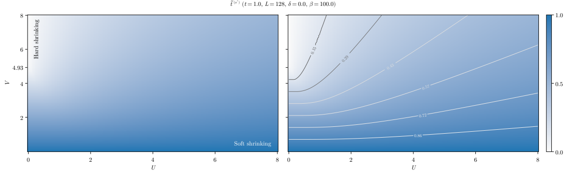
Figure 5.7 | Numerical results for the HFP u^{(s*)} . In the left panel we indicate the converged value of u^{(s*)} in the bottom-left corner. In the right panel we plot isovalues.
