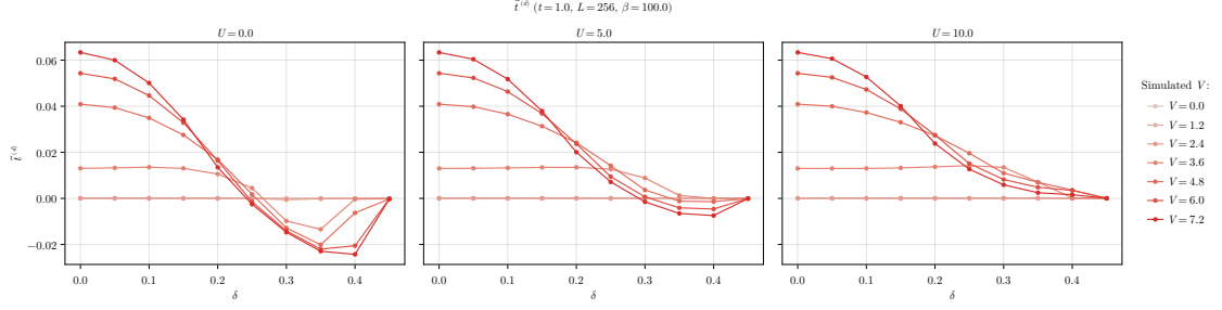
b | Dependency of \tilde{t}^{(d)} on \delta at various V s, compared at three values of U .
