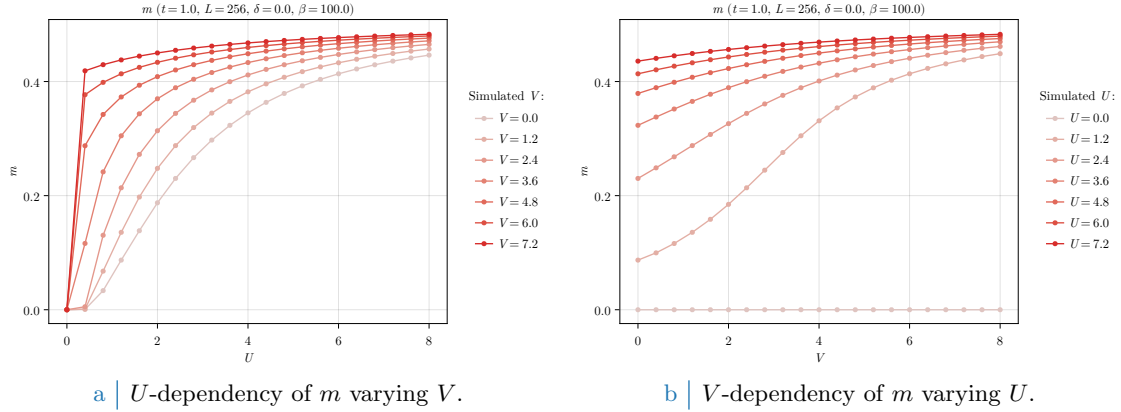
Figure 5.11 | Plot of the self-consistent convergence values for the HFPs m and u^{(s^*)} in the AF phase.
