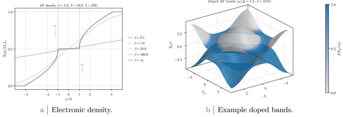
Figure 5.3 Left panel: electronic density in the AF phase as a function of the chemical potential, computed through Eq. (5.52), at various temperatures. Right panel: example doped bands, with \mu/\Delta = 1.5 set arbitrarily and temperature set to \beta = 10 to enhance smearing effects around the FS. Single-state filling is proportional to the colour intensity.
