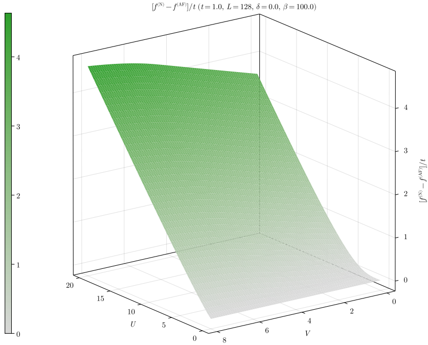
Figure 5.13 | Difference of free energies for the normal phase minus the AF phase.
