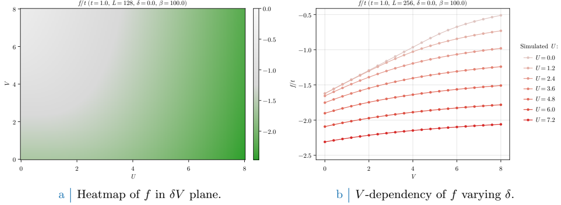
Figure 5.12 | Free energy density of the AF phase.
