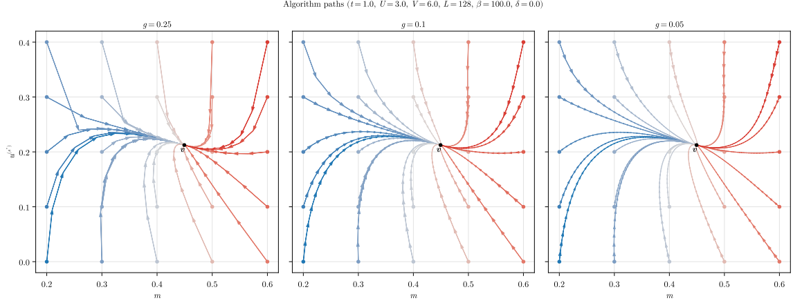
Figure 5.14 | Quiver plot of algorithmic evolution in HFPs space at fixed model parametrisation. The black dot \mathbf{v} represents the nonlinear map fixed point, while the colored paths the sequences of HFPs coordinates simulated via iterative HF procedure, starting from different HFPs initialisers (colored dots).
