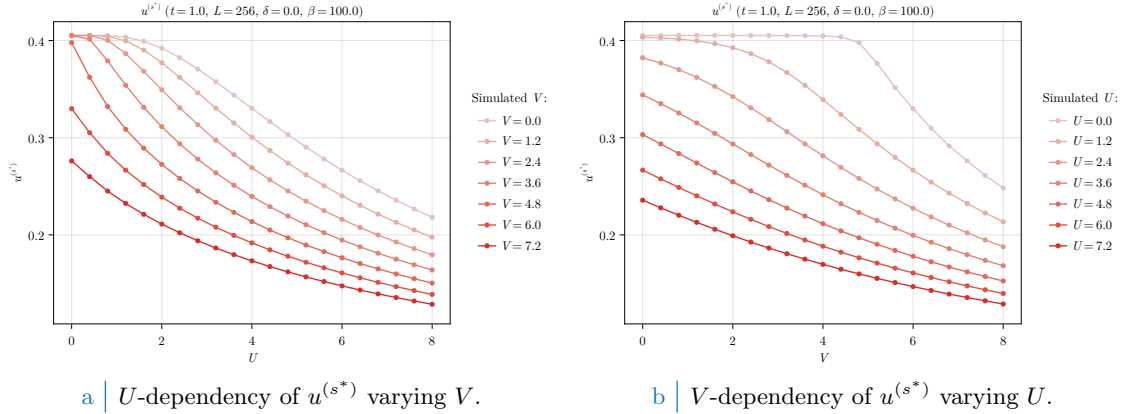
Figure 5.6 | Plot of the self-consistent convergence values for the HFPs m and u^{(s*)} in the AF phase.
