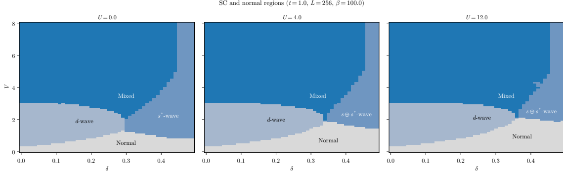
Figure 4.5 | Depiction of the normal state region and the three singlet superconducting regions, at U/t = 0, 4, 12 from left to right. Lighter blue indicates the pure d -wave SC phase, blue the isotropic s \oplus s^* phase, deeper blue the mixed region. In text is described the convention we used to identify the boundaries.
