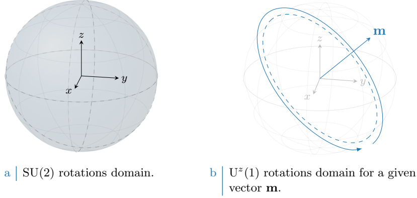
Figure 1.2 | Graphic representation of the domain of SU(2) rotations (left figure) and U^z(1) rotations (right figure). For any given direction \mathbf{m} , the group of rotations around said direction is contained in the larger group SU(2).
