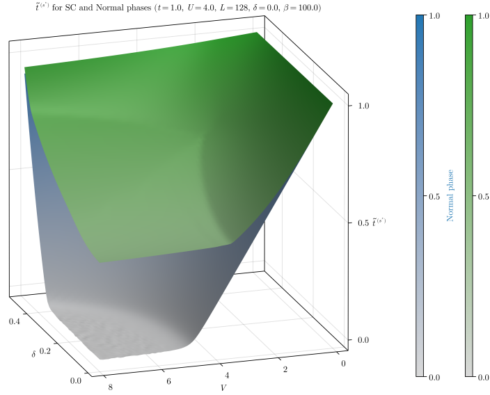
Figure 4.9 | Comparison of the isotropic part of the renormalised hopping \tilde{t}^{(s^*)} for the SC (green) and normal (blue) phases on the (\delta, V) plane. The data from the normal phase are the same of Fig. 2.6.
