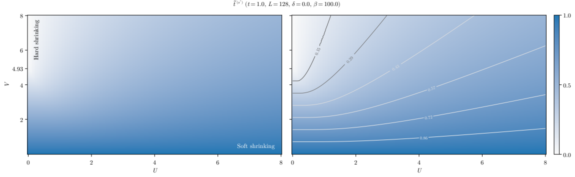
Figure 3.7 | Numerical results for the HFP u^{(s*)} . In the left panel we indicate the converged value of u^{(s*)} in the bottom-left corner. In the right panel we plot isovalued lines.
