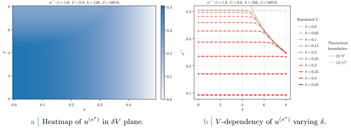
Figure 2.5 | Numerical results for u^{(s^*)} . On the left: colour plot in the (\delta, V) plane. On the right: line plot at doubled lattice size, varying \delta . The theoretical value for u^{(s^*)} computed in Eqs. (2.48) at half-filling is plotted as a green dashed line.
