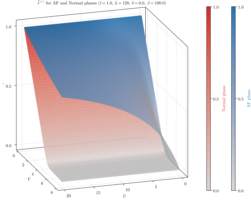
Figure 3.9 | Comparative plot of the converged values for \tilde{t}^{(s^*)} for the normal phase and the AF phase.
