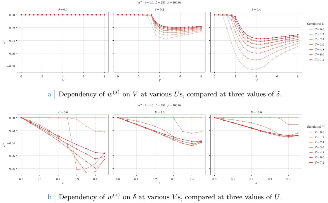
Figure 4.1 | Dependency of the s -wave HFP w^{(s)} on V at fixed U and \delta (top panel, compared figures) and on \delta at fixed V and U (bottom panel, compared figures).
