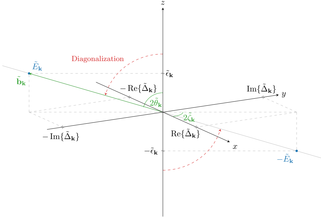
Figure 3.4 Sketch of the diagonalisation procedure for the EHM antiferromagnet. To diagonalise the HF hamiltonian, we align the z axis with the pseudo-field. This is an extension of Fig. 3.2.
