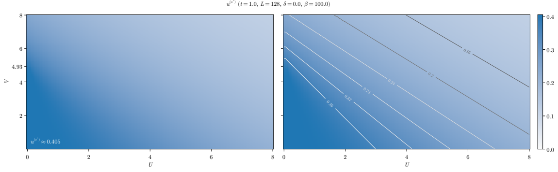
Figure 3.5 | Numerical results for the HFP u^{(s*)} . In the left panel we indicate the converged value of u^{(s*)} in the bottom-left corner. In the right panel we plot isovalues lines.
