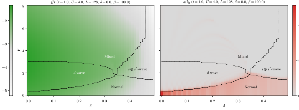
Figure 4.10 Heatmaps of the free energy and entropy densities at U/t = 4 . The black dotted lines represent the internal boundaries of the singlet SC phase, extracted from Fig. 4.5.
