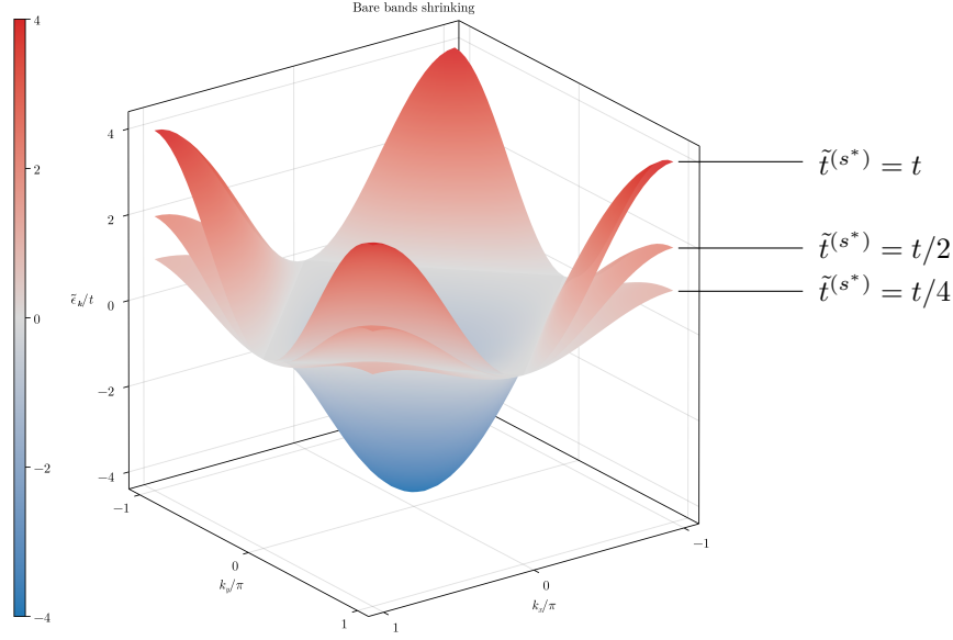
Figure 2.3 | Graphic representation of the shrinking of renormalised band \tilde{\epsilon}_{\mathbf{k}} = -4t\varphi_{\mathbf{k}}^{(s^*)} , as the hopping parameter is decreased by renormalisation.
