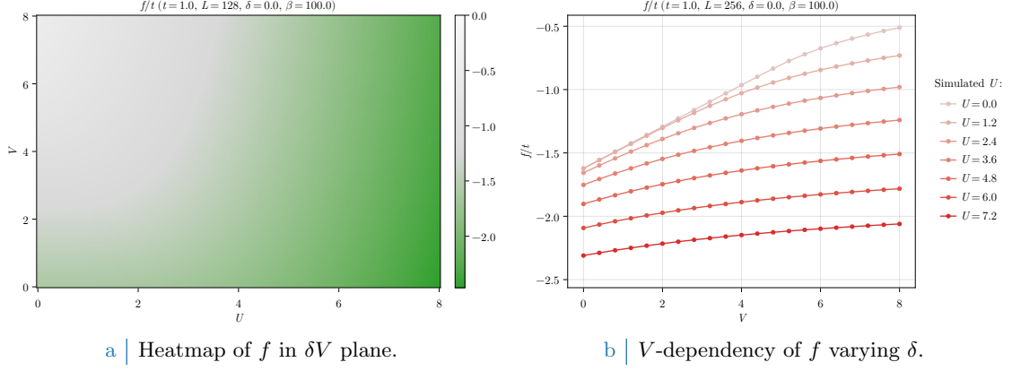
Figure 3.12 | Free energy density of the AF phase.
