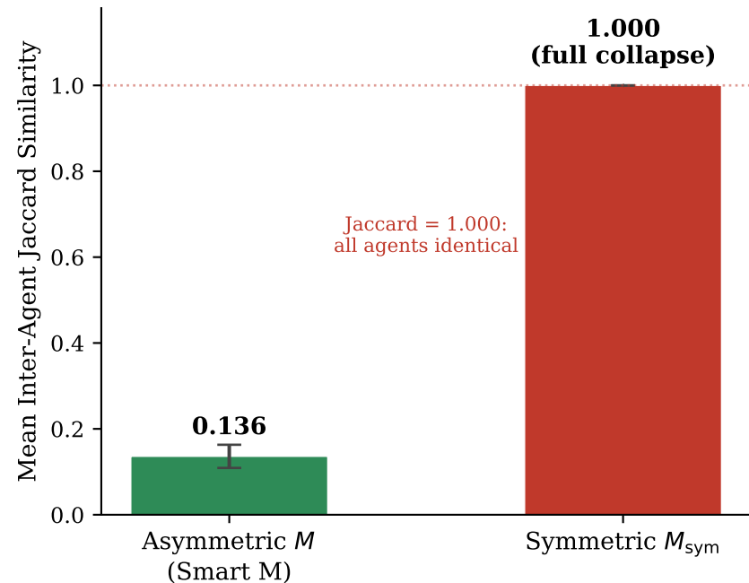
(a) Diversity Collapse Under Symmetric M
