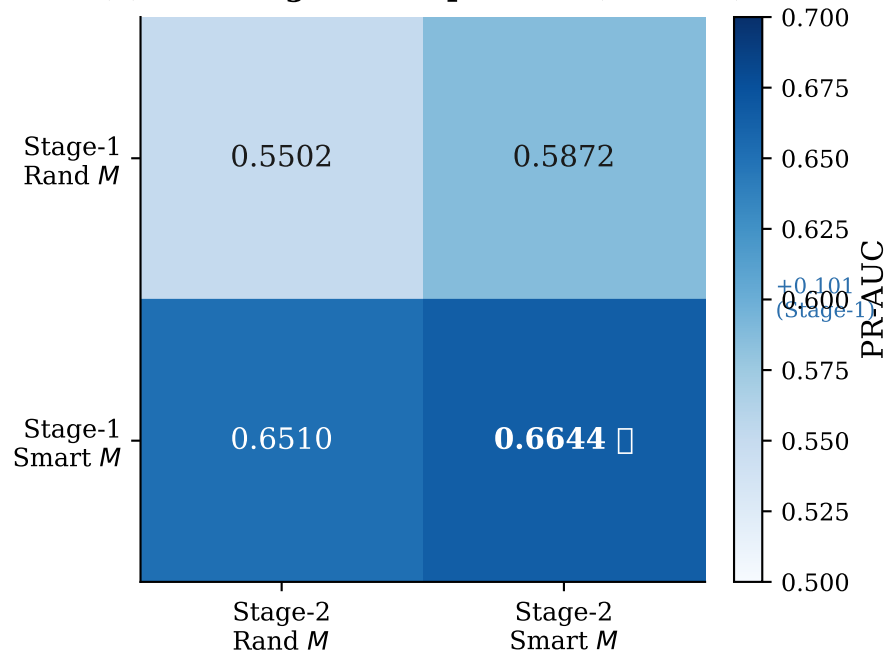
(b) 2×2 Stage Decomposition (PR-AUC)
