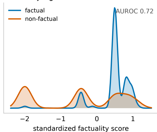
LLM-judge score — Llama-3.1-8B
